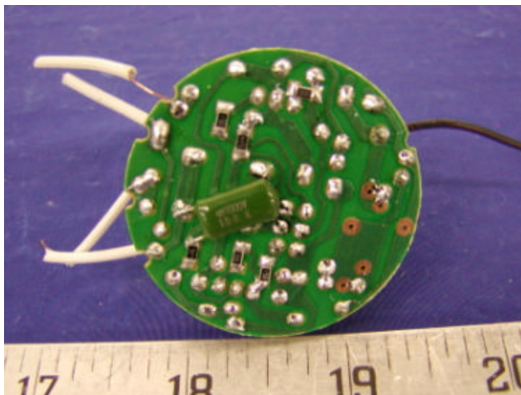
EUT – AF15W Solder View
