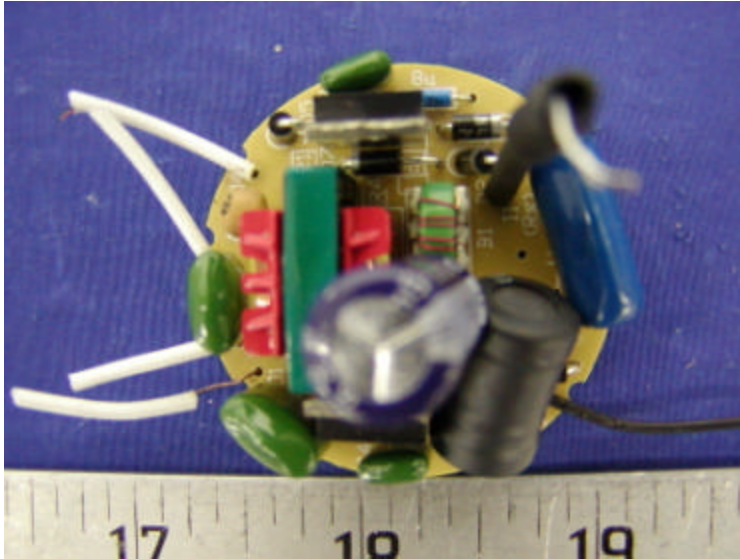
EUT – AF15W Component View
