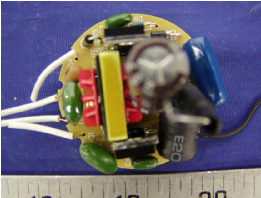
EUT – AF25W Component View
