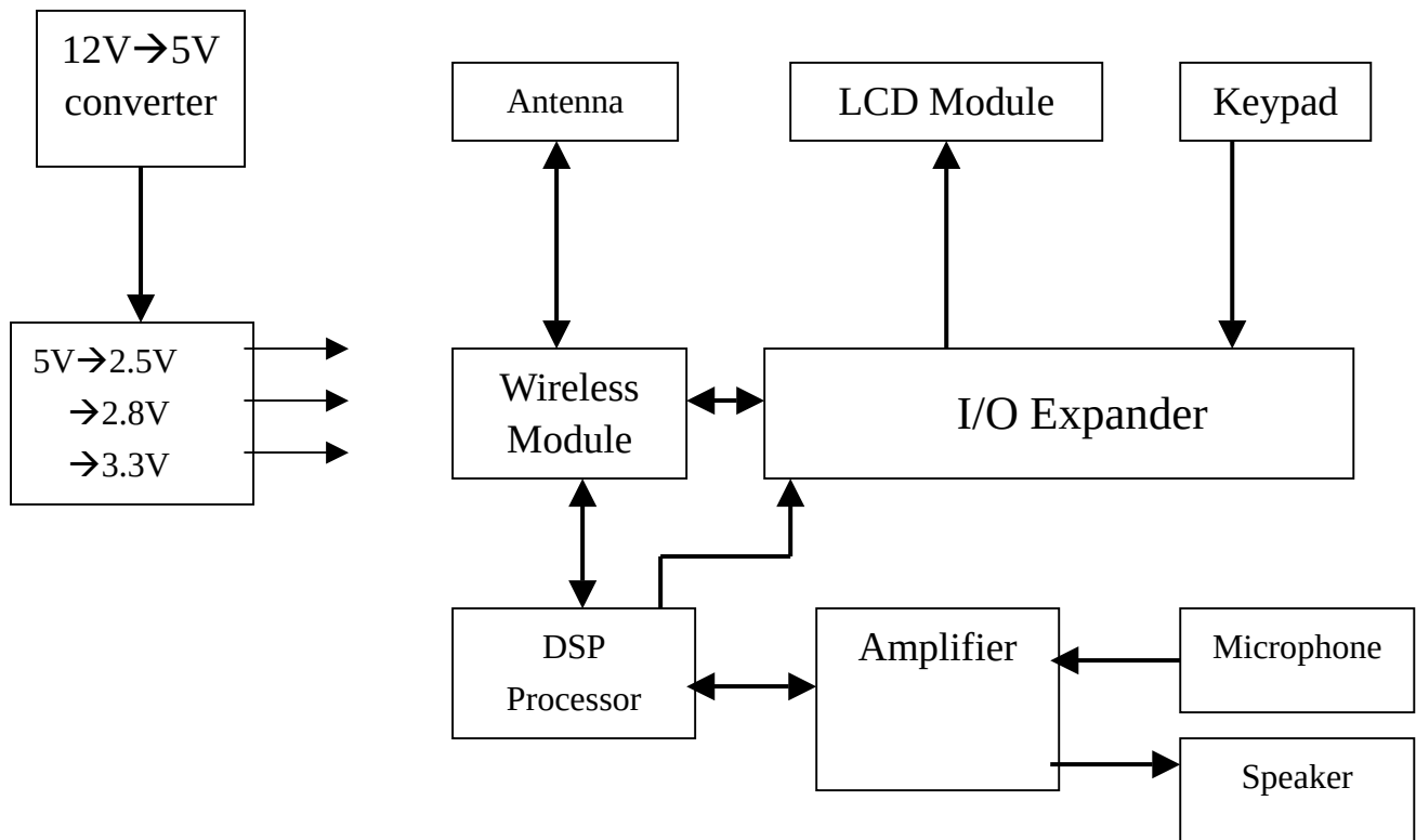
Car Kit Block diagram:
