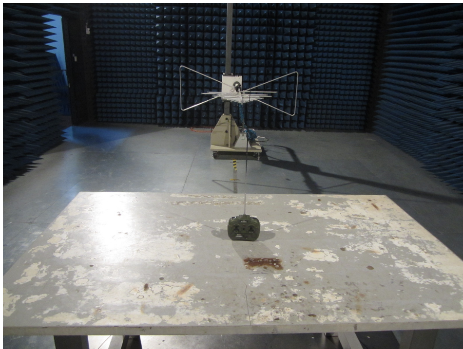
Set-up of Radiation Emission from 30 – 1000MHz
