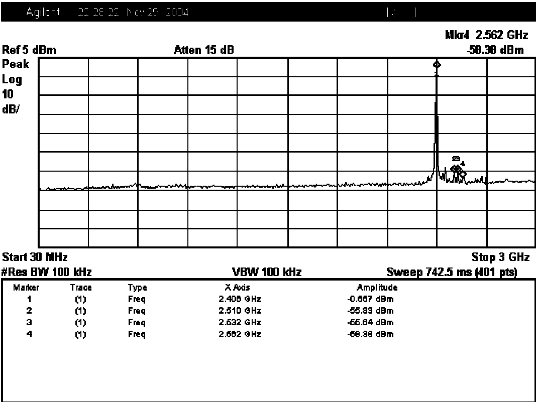
Figure 6. Plot of the RF antenna port emissions (Conducted) Lowest Channel (operating at 2402 MHz): 30MHz ~ 3GHz
