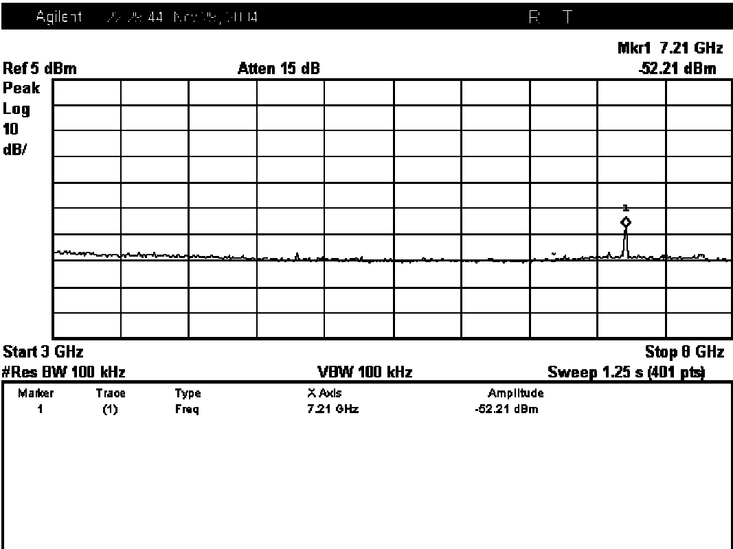
Lowest Channel (operating at 2402 MHz): 3GHz ~ 8GHz
