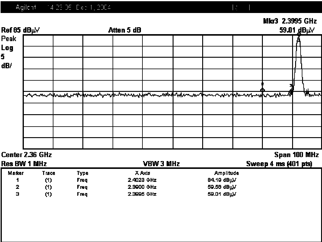
Figure 8. Plot of the Band Edge (Radiated) Lowest Channel (operating at 2402 MHz): 2310 ~ 2390 MHz
