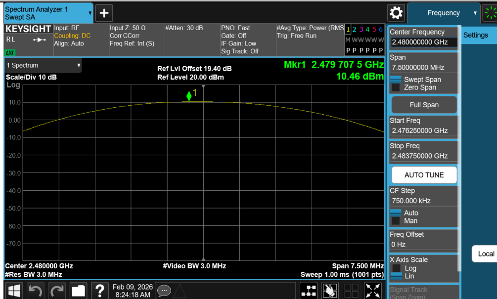
DH5-Ant1-2480-PASS
