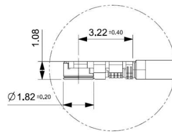
DETAIL B SCALE 8:1 CONNCTOR
