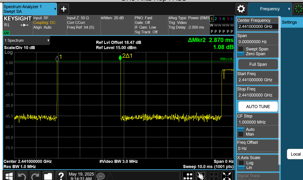
DH5-Ant1-Hop-PASS
