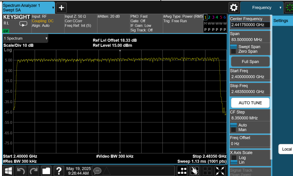
3DH5-Ant1-Hop-PASS
