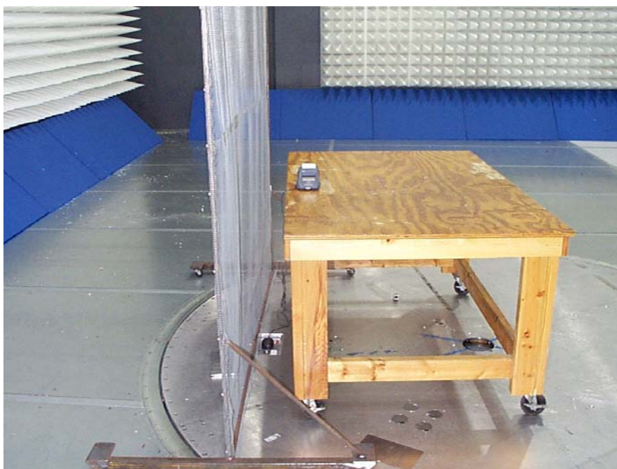
Figure 2-6: Conducted Voltage Emissions (Side)
