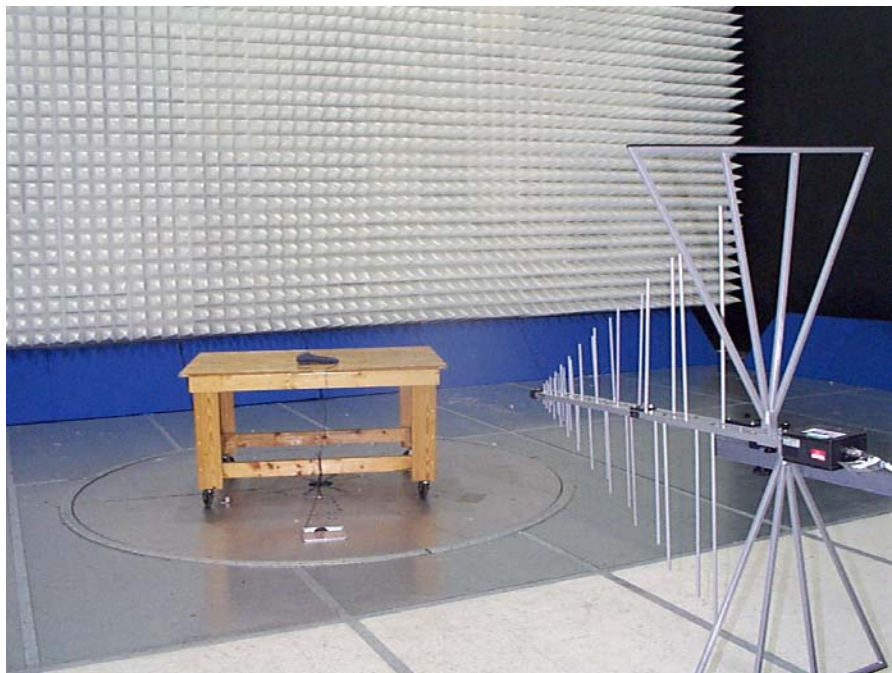
Figure 2-3: Spurious Emissions (Horizontal Orientation Bilog Antenna)
