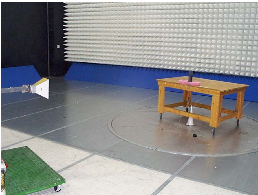
Figure 2-1: EIRP Testing (Vertical Orientation)
