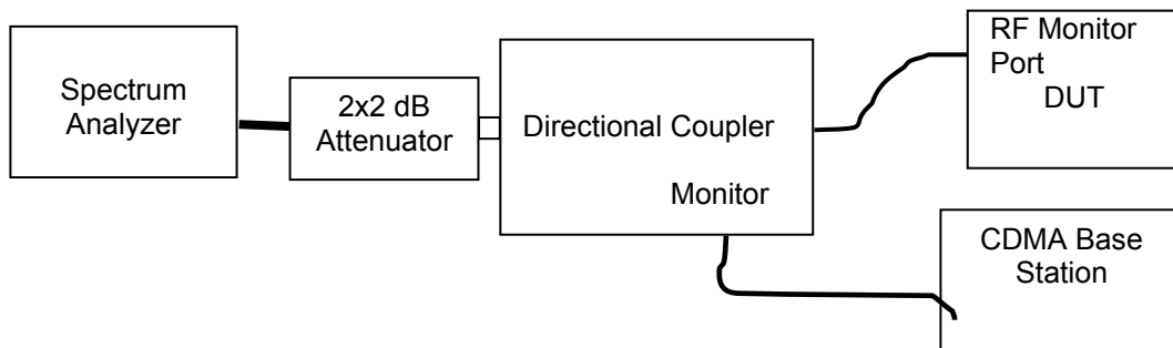
Figure L.6-1 - Setup Drawing
