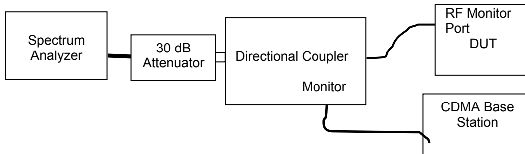
Figure B.6-1 - Setup Drawing
