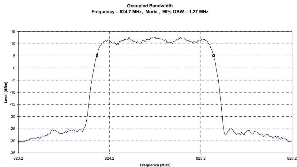
Channel 1013 (824.70 MHz)
