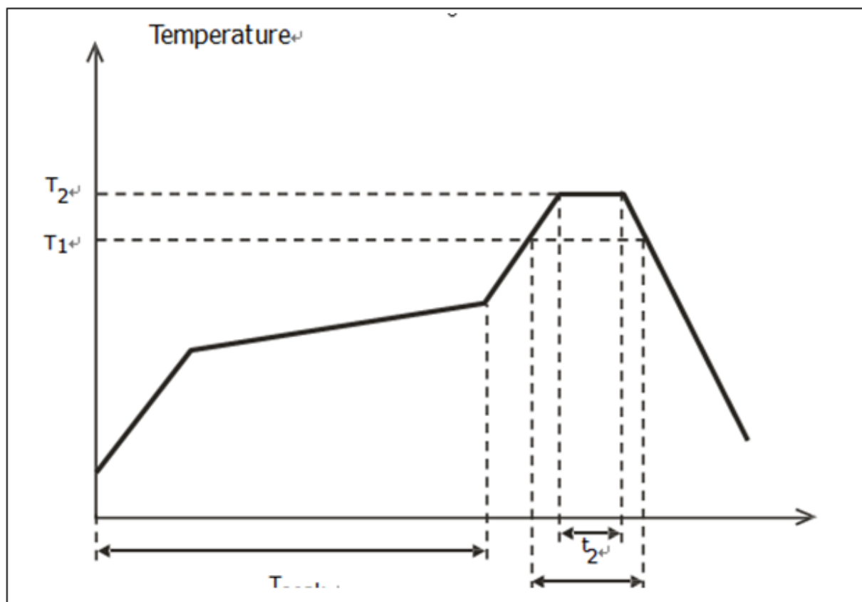
FIGURE 10-1: REFLOW PROFILE
