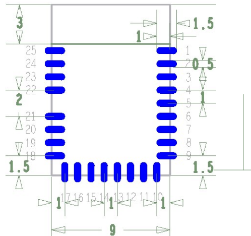
Figure 2 Physical dimensions and pinout (mm) – Top view
