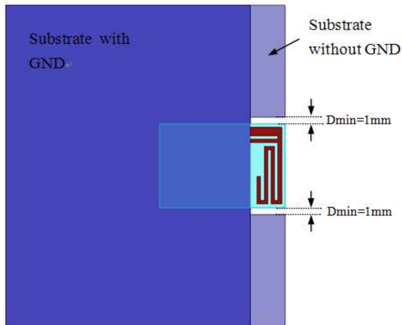
Figure 5 Layout when any dielectric material around antenna
