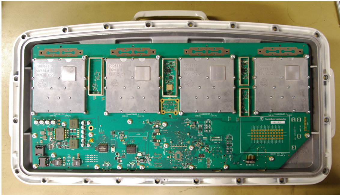
3 GHz PMP 450m Integrated Access Point, PCB in Enclosure with RF Shields
