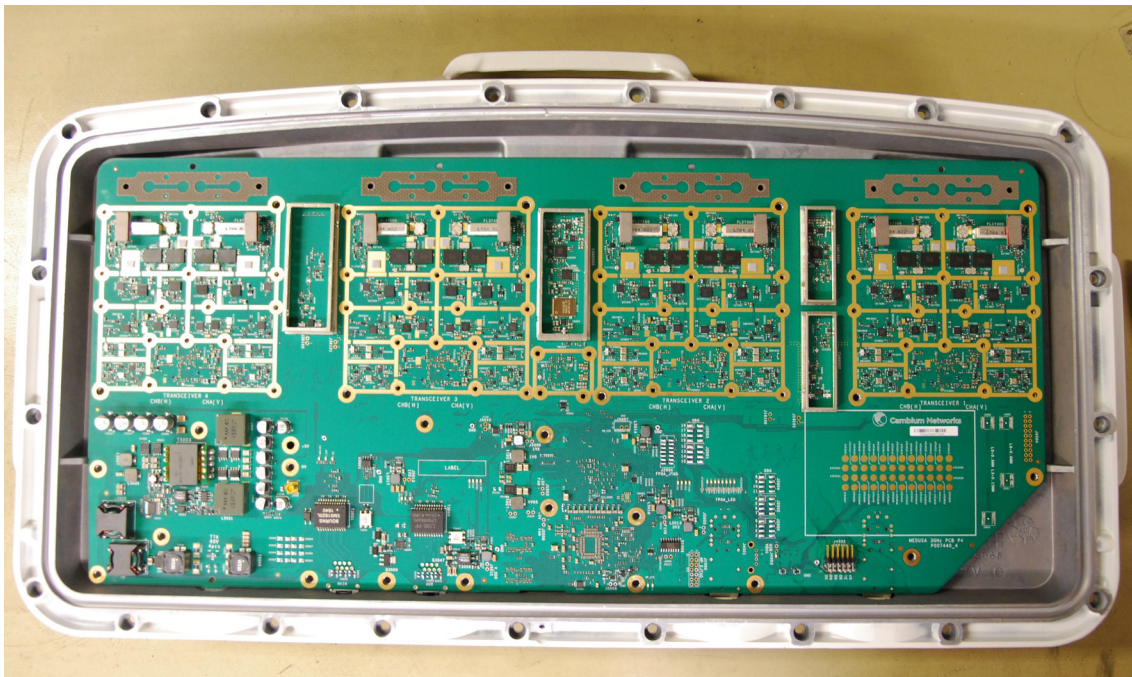
3 GHz PMP 450m Integrated Access Point, PCB in Enclosure with RF Shields
