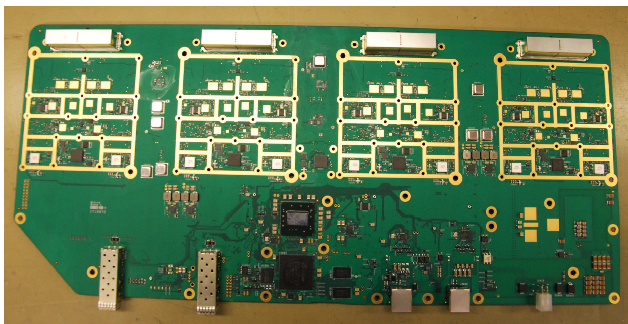
3 GHz PMP 450m Integrated Access Point, Bottom of PCB No Shields
