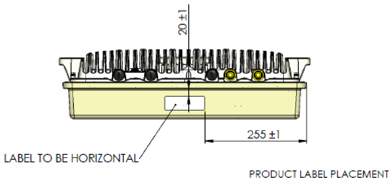
3 GHz PMP 450m Integrated Access Point, Label Location
