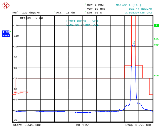
Emission Mask 256 QAM; 3697.5 MHz; MIMO A.
