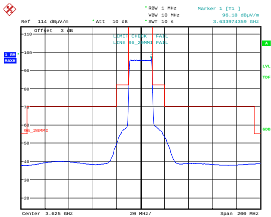
Date: 14.AUG.2018 22:29:19 Emission Mask 16 QAM; 3625 MHz; MIMOB.
