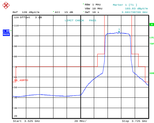
Emission Mask 256 QAM; 3680 MHz; MIMO B.
