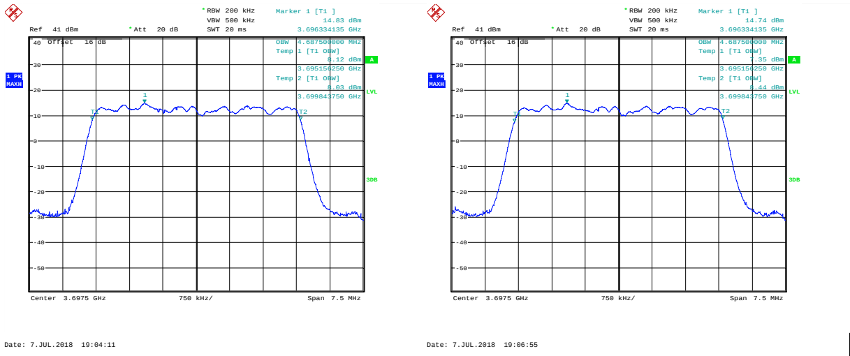
99 % Bandwidth; 16QAM; 3697.5 MHz; MIMO A.
