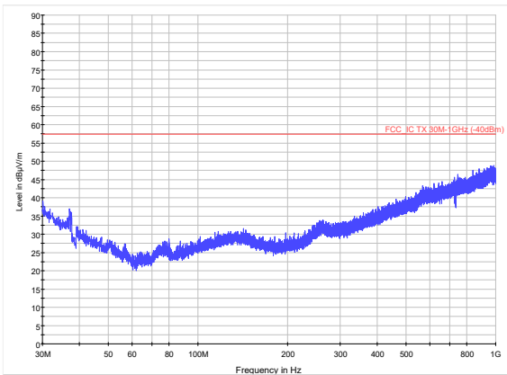
30 MHz to 1 GHz; Beamform; QPSK; MIMO.A.
