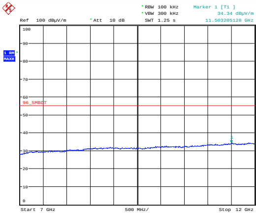
7 GHz to 12 GHz; Beamform; QPSK; MIMO.A.
