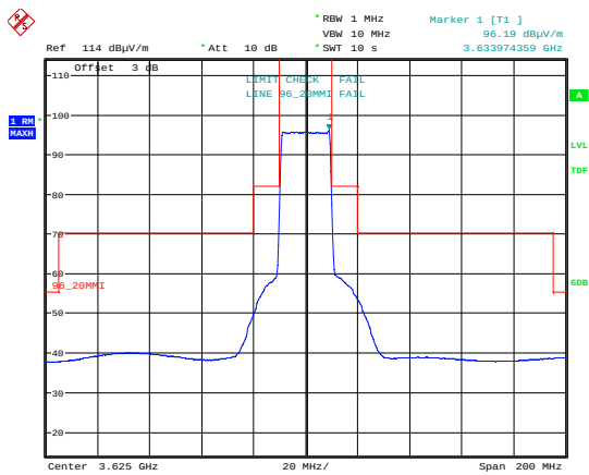
Date: 14.AUG.2018 22:21:10 Emission Mask 64 QAM; 3625 MHz; MIMO A.
