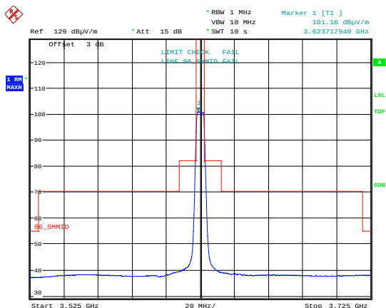
Date: 14.AUG.2018 18:10:12 Emission Mask 64 QAM; 3625 MHz; MIMOB.
