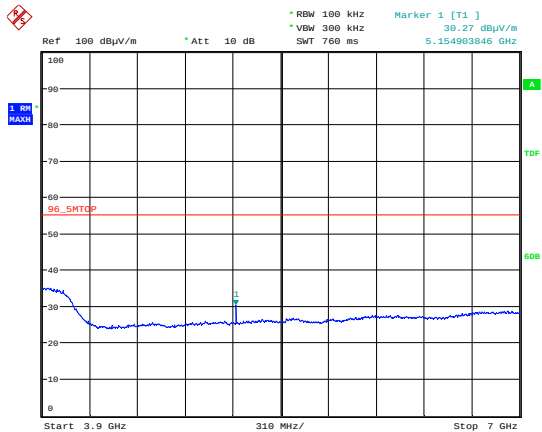
3.9 GHz to 7 GHz; Beamform; QPSK; MIMO.A.
