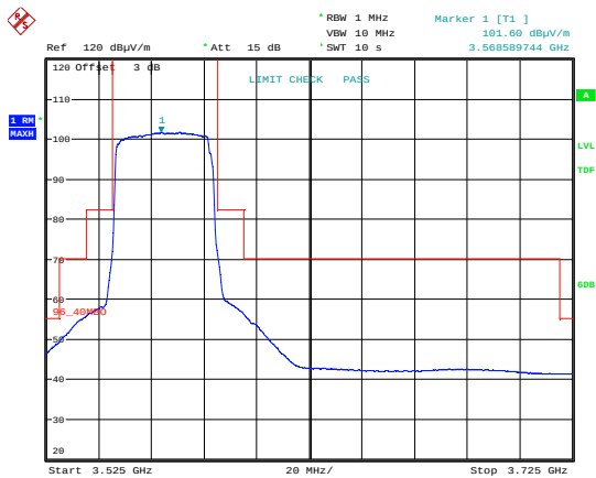
Emission Mask 256 QAM; 3570 MHz; MIMO A.
