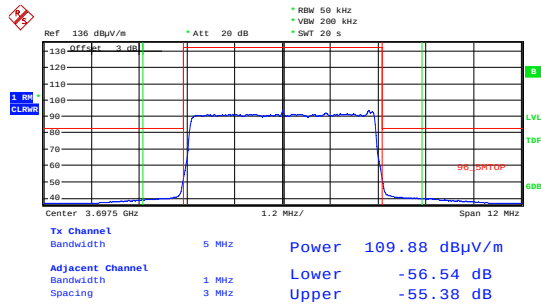
Emission Mask 64 QAM; 3697.5 MHz; MIMO A Integration Method.
