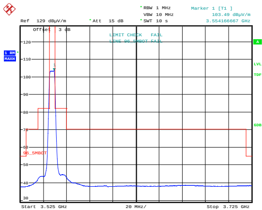
Emission Mask 256 QAM; 3552.5 MHz; MIMO A.
