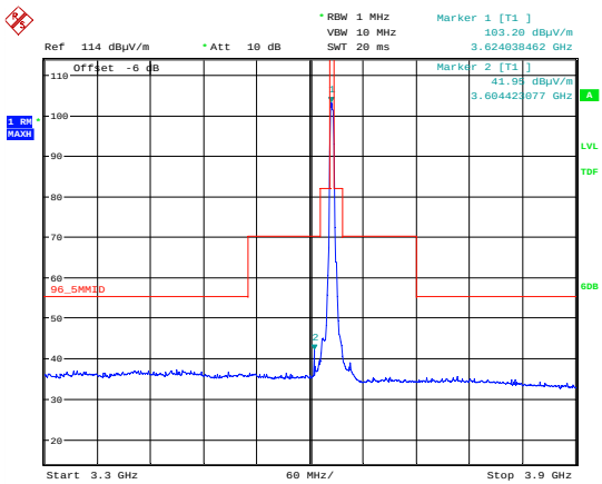
3.3 GHz to 3.9 GHz; Beamform; QPSK; MIMO.A.
