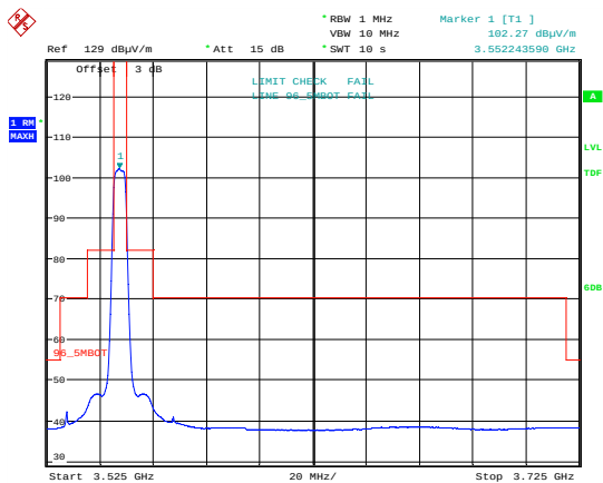
Emission Mask 64 QAM; 3552.5 MHz. MIMOB
