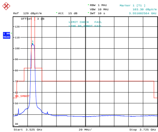
Emission Mask 64 QAM; 3552.5 MHz; MIMO A.
