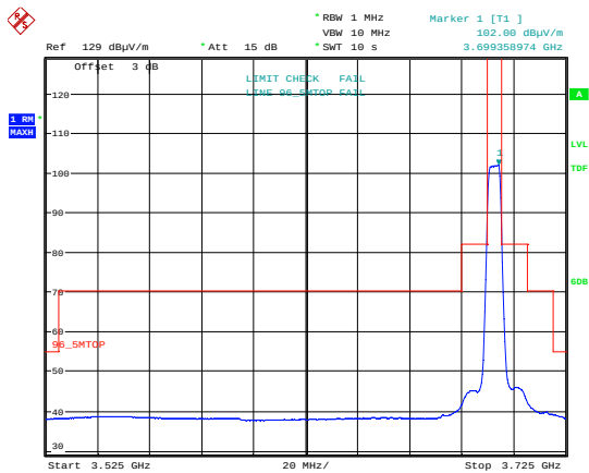
Emission Mask 16 QAM; 3697.5 MHz; MIMOB.
