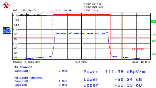
Emission Mask 64 QAM; 3552.5 MHz; MIMO A Integration Method.
