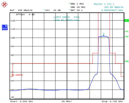
Emission Mask 16 QAM; 3690 MHz; MIMOB.
