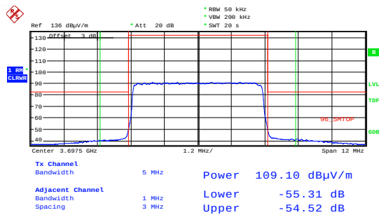
Emission Mask 16 QAM; 3697.5 MHz; MIMOB Integration Method.
