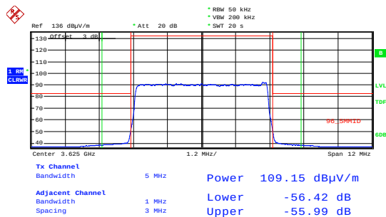
Date: 14.AUG.2018 18:03:39 Emission Mask 64 QAM; 3625 MHz; MIMOA Integration Method.
