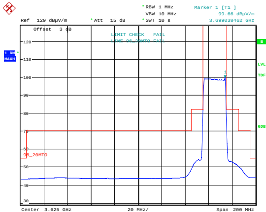
Emission Mask 256 QAM; 3690 MHz; MIMO A.
