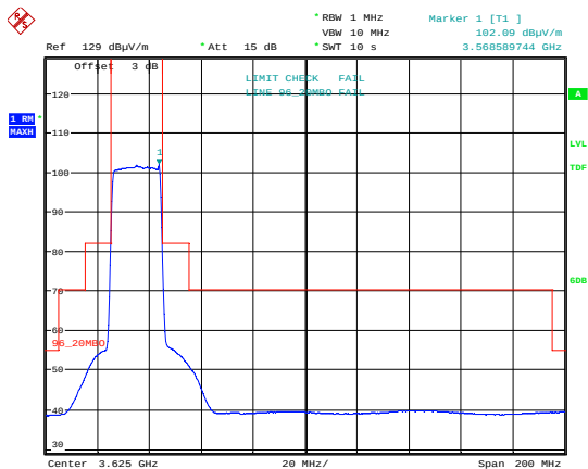
Emission Mask 256 QAM; 3560 MHz; MIMO A.
