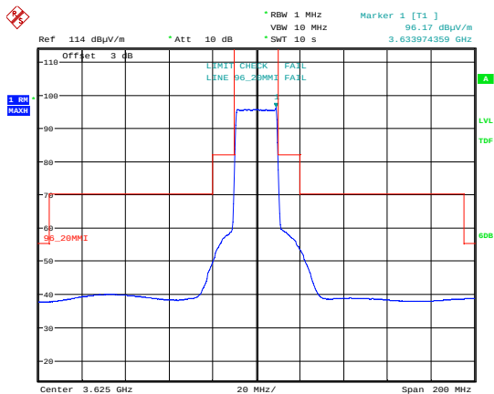
Emission Mask 256 QAM; 3625 MHz; MIMO A.
