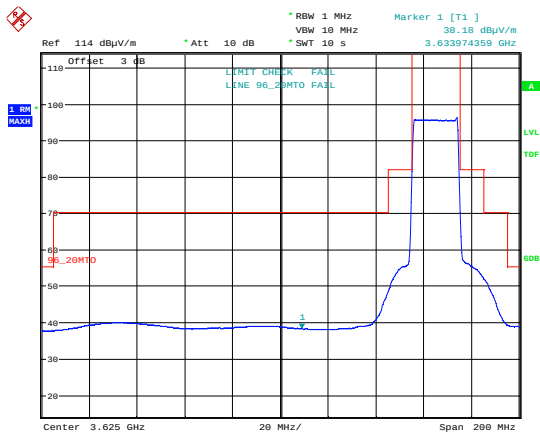
Emission Mask 256 QAM; 3690 MHz; MIMO B.
