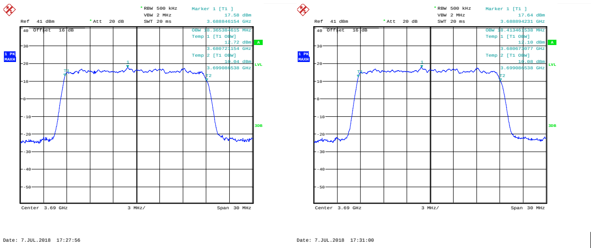
99 % Bandwidth; 16QAM; 3690 MHz; MIMO A.
