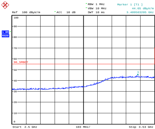
2.5 GHz to 3.53 GHz; Beamform; QPSK; MIMO.A.
