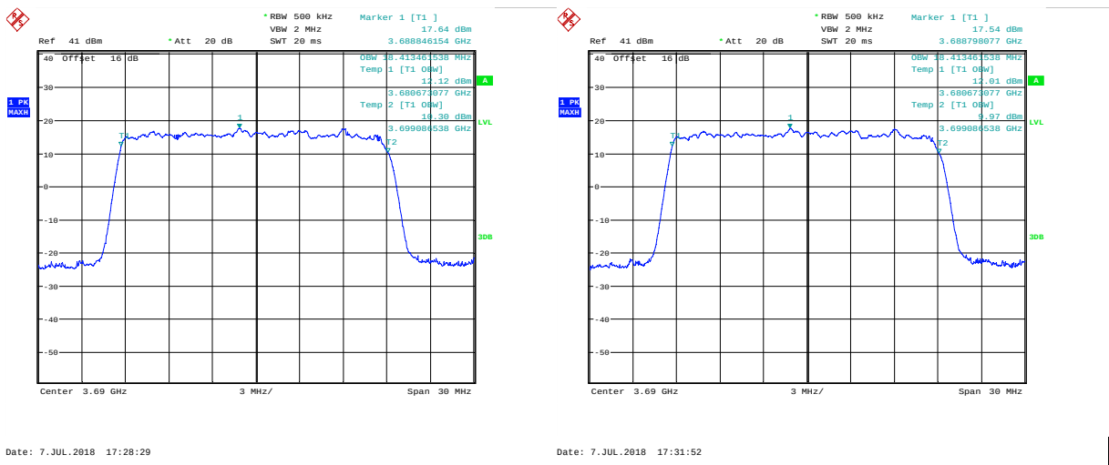
99 % Bandwidth; 64QAM; 3690 MHz; MIMO A.
