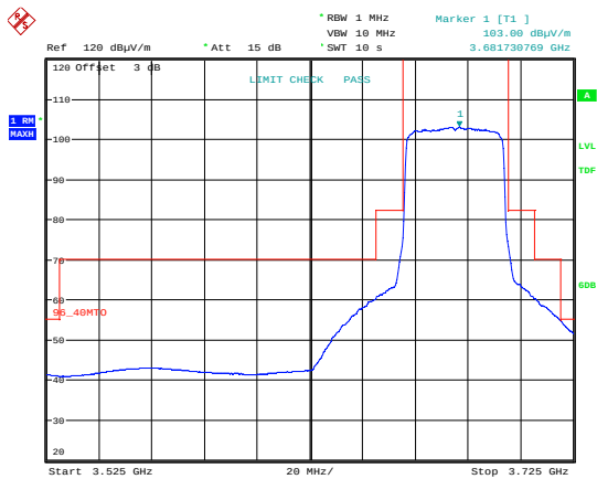
Emission Mask 256 QAM; 3680 MHz; MIMO A.
