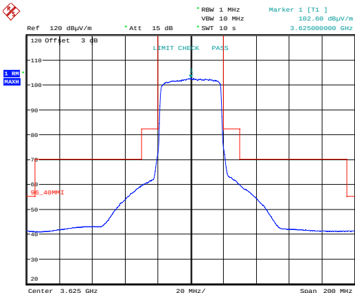
Emission Mask 16 QAM; 3625 MHz; MIMO A.
