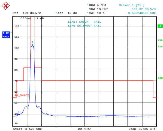
Emission Mask 16 QAM; 3552.5 MHz. MIMOB
