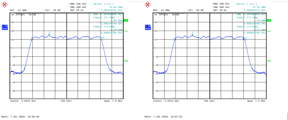
99 % Bandwidth; 64QAM; 3697.5 MHz; MIMO A.
