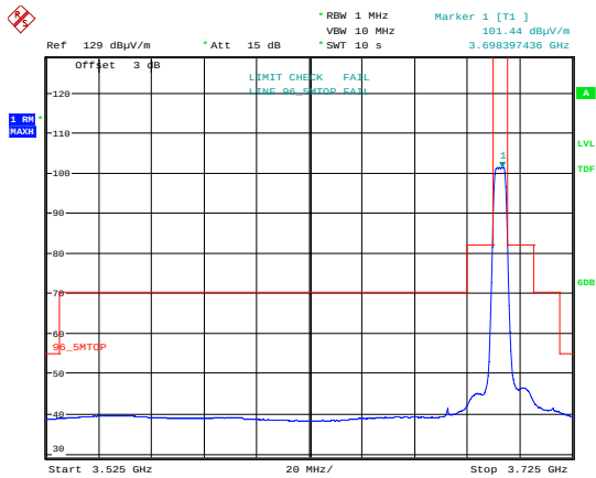
Emission Mask 64 QAM; 3697.5 MHz; MIMOB.
