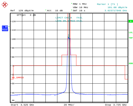
Date: 14.AUG.2018 18:08:53 Emission Mask 16 QAM; 3625 MHz; MIMOB.
