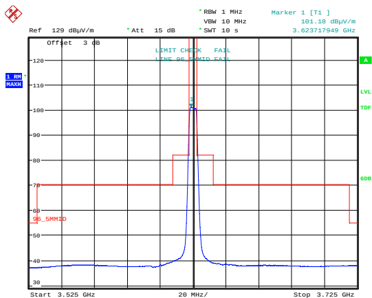
Date: 14.AUG.2018 18:03:08 Emission Mask 64 QAM; 3625 MHz; MIMOA.
