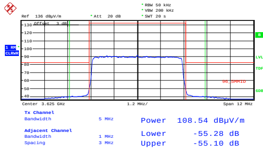
Emission Mask 64 QAM; 3625 MHz; MIMOA Integration Method.
