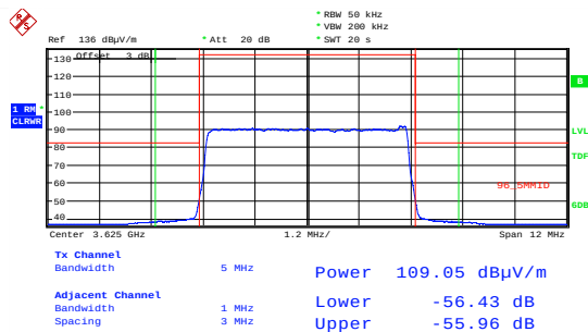
Date: 14.AUG.2018 18:17:17 Emission Mask 16 QAM; 3625 MHz; MIMOB Integration Method.
