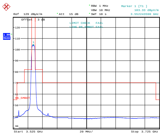
Emission Mask 16 QAM; 3552.5 MHz; MIMOB.
