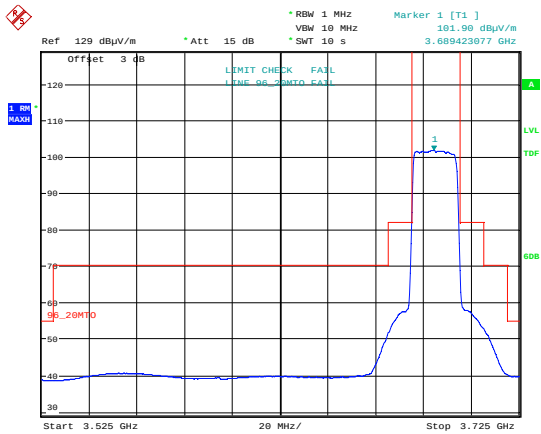
Emission Mask 64 QAM; 3690 MHz; MIMOB.
