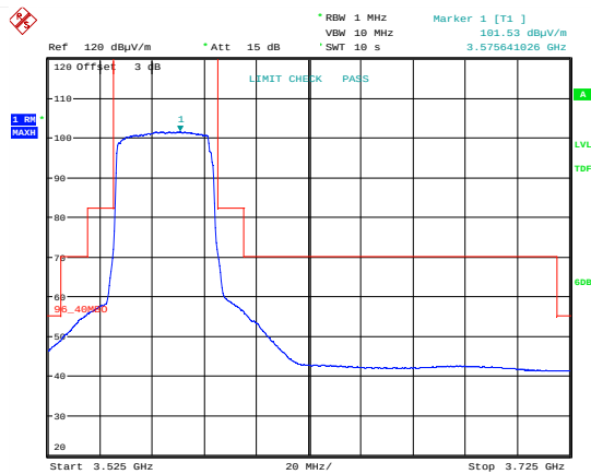
Emission Mask 256 QAM; 3570 MHz; MIMO B.
