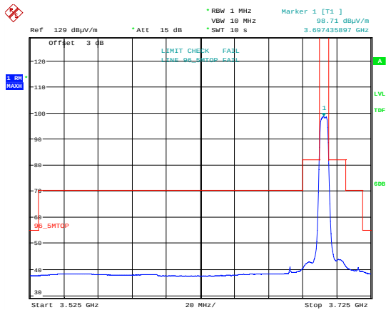
Emission Mask 64 QAM; 3697.5 MHz. MIMOA
