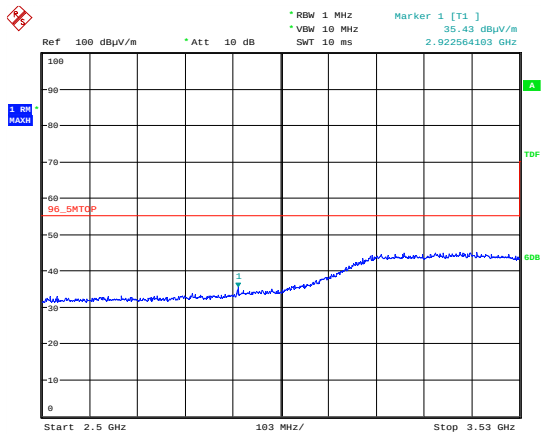
2.5 GHz to 3.53 GHz; Beamform; QPSK; MIMO.A.
