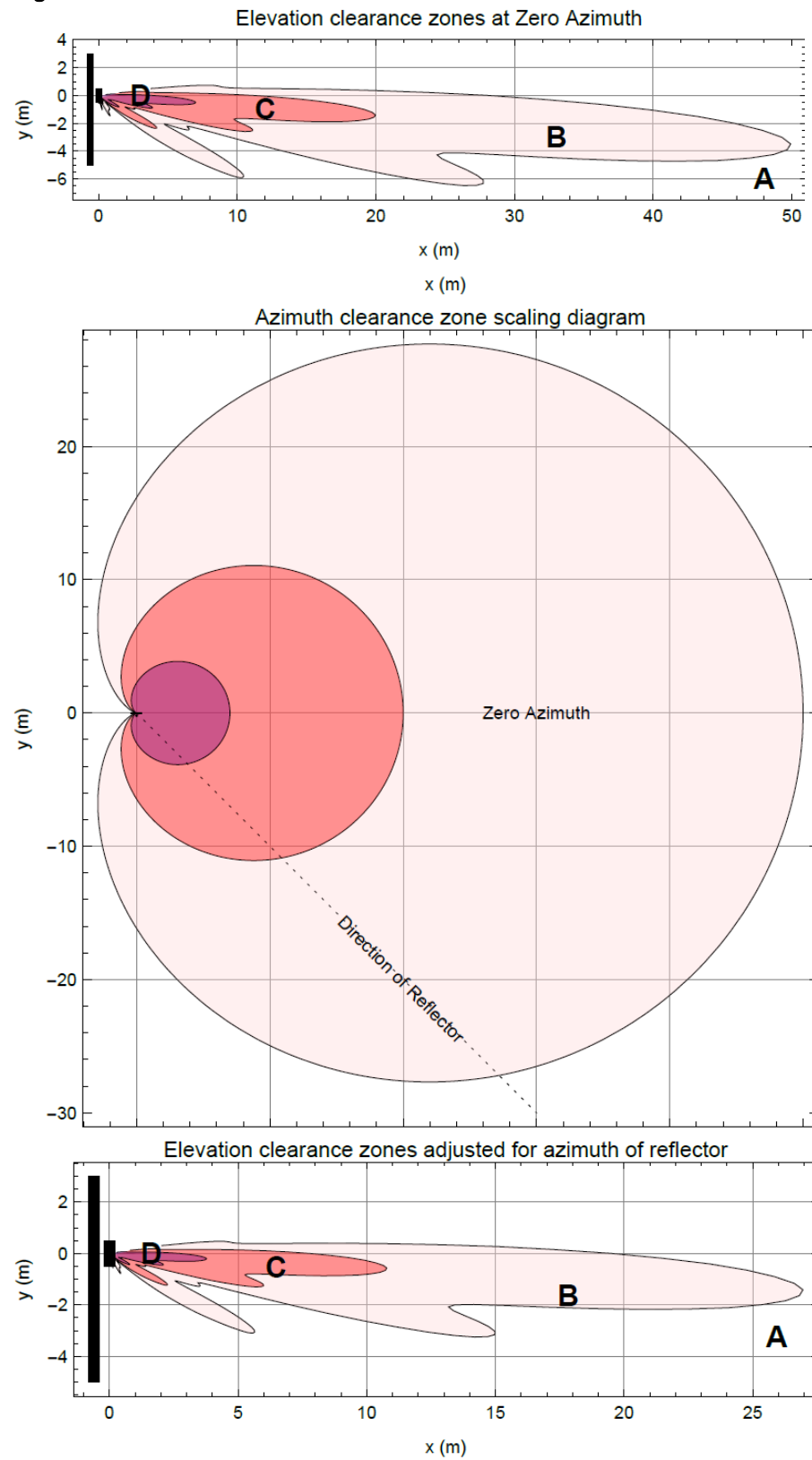
Figure 55 Sector Antenna
