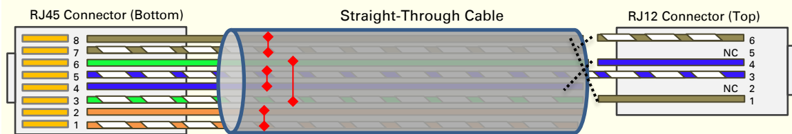
Figure 73 AP/BHM to UGPS cable
