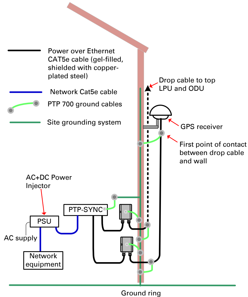
Figure 42 GPS receiver wall installation
