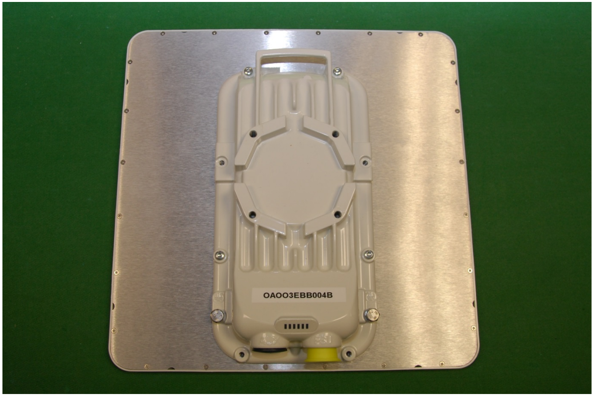
PMP 450i / PTP 450i Rear View – Integrated Subscriber Module and PTP ODU
