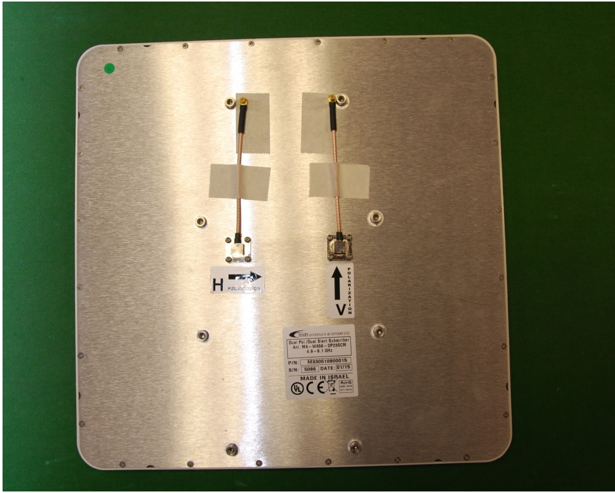
PMP 450i / PTP 450i Rear View – Subscriber Module and PTP ODU Integrated Directional Antenna
