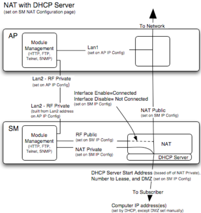
Figure 136 NAT with DHCP server implementation
