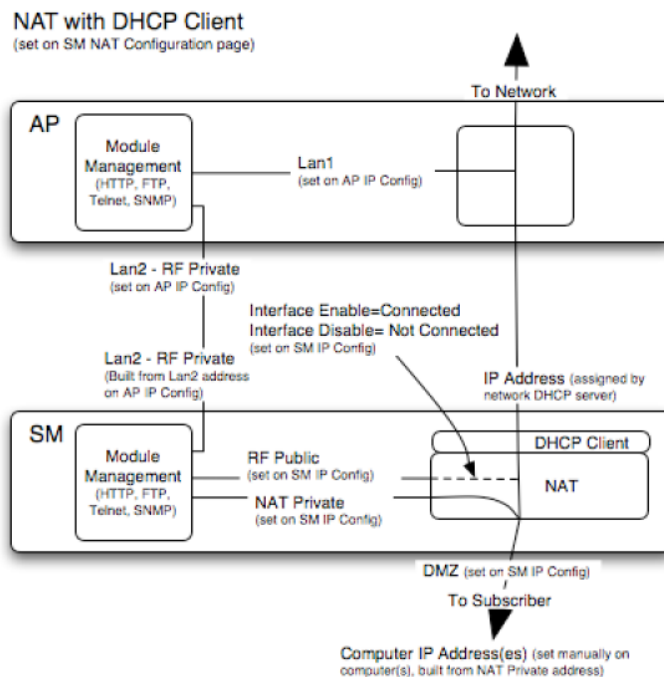
Figure 135 NAT with DHCP client implementation
