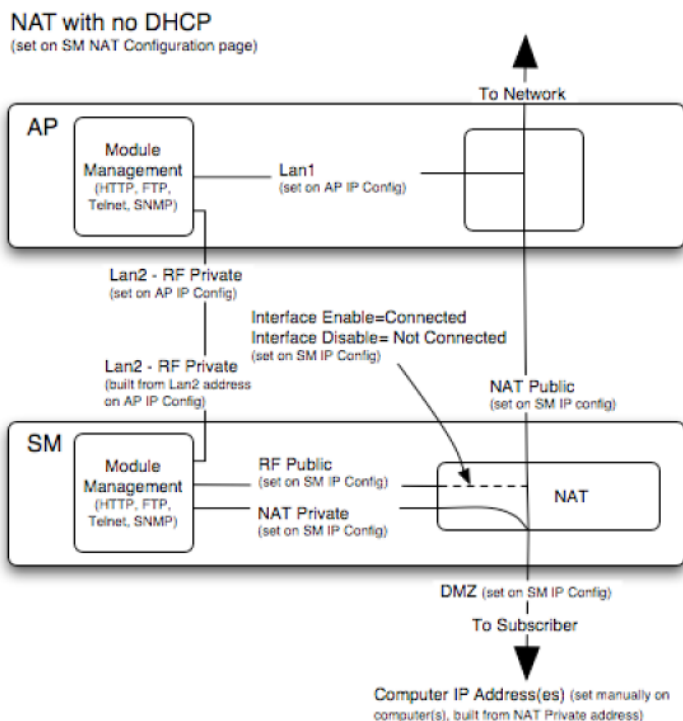
Figure 137 NAT without DHCP implementation
