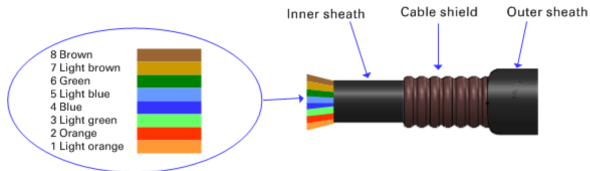
Figure 23 Outdoor drop cable
