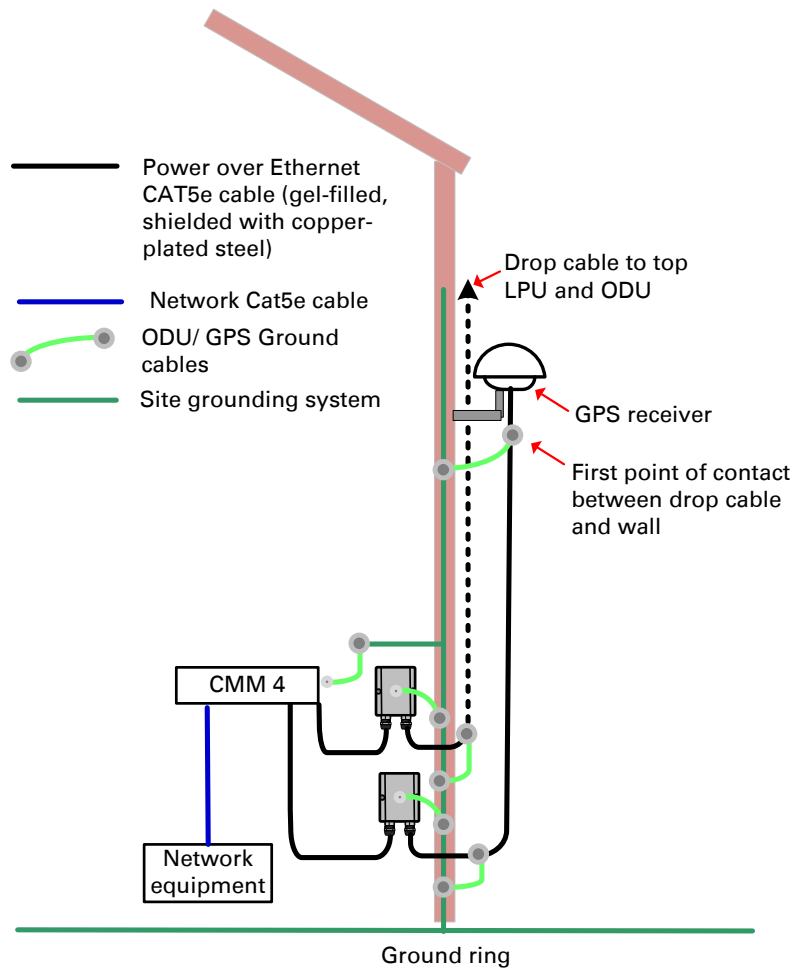
Figure 45 GPS receiver wall installation
