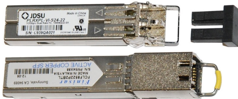
Figure 24 Optical SFP transceiver module
