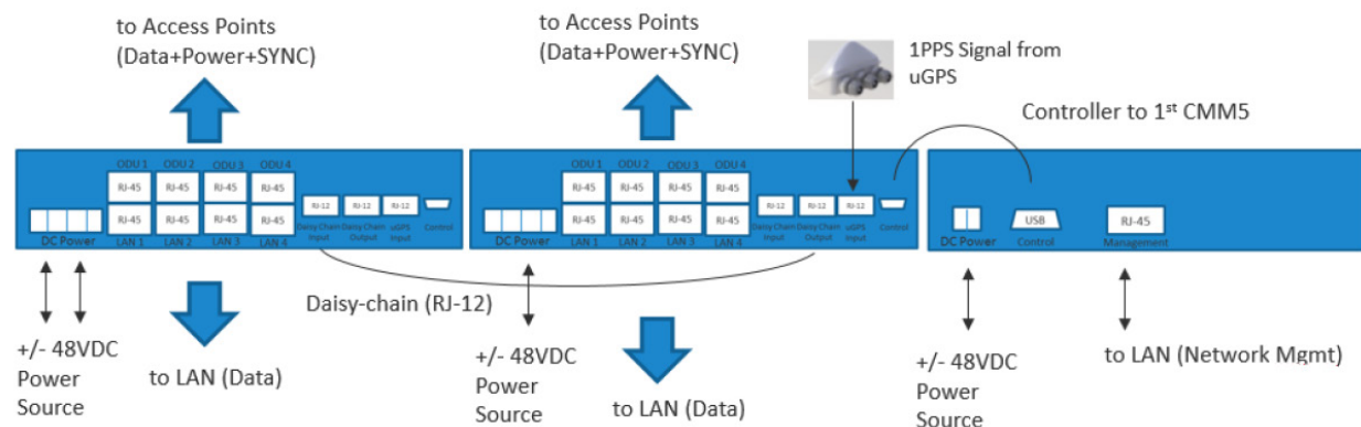
Figure 32 Cluster Management: Scenario 2
