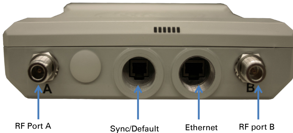
Figure 6 PMP/PTP 450 Series - AP interfaces
