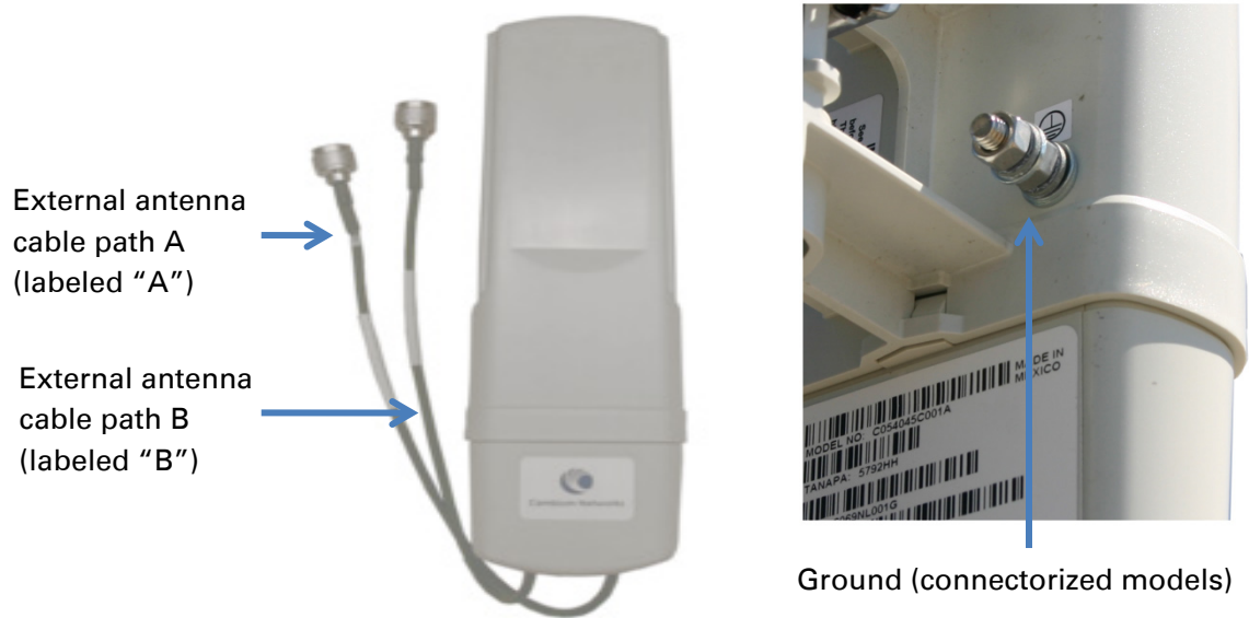
Figure 8 PMP/PTP 450 Series – SM/BH Connectorized interfaces
