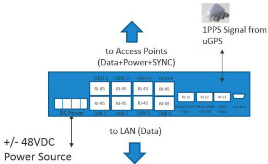
Figure 31 Cluster Management: Scenario 1
