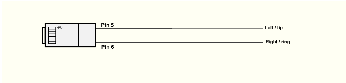
Figure 27 RJ12 Alignment Tone Cable
