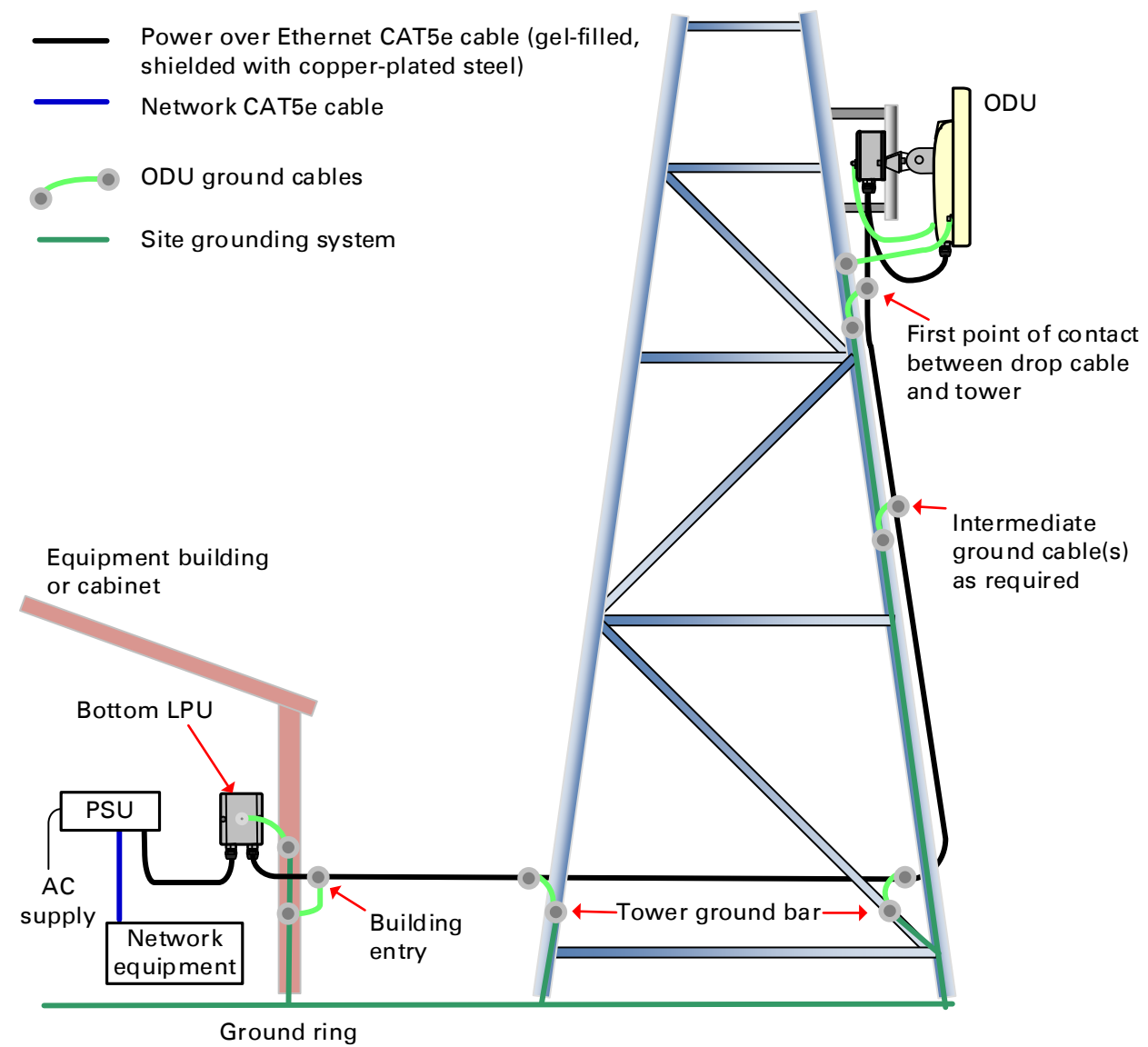
Figure 42 Mast or tower installation
