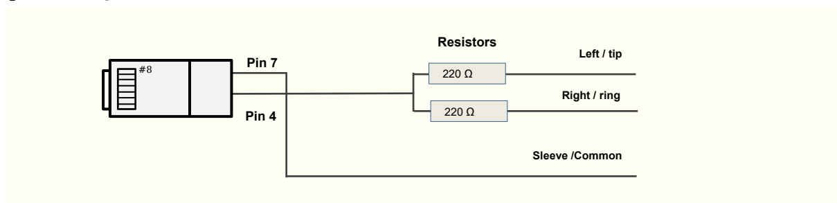
Figure 26 Alignment Tone Cable
