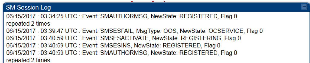
Figure 206 SM Session log
