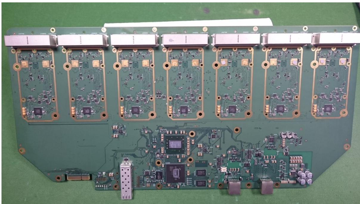
PMP 450m PCB A005138 Rear View (with RF Shields Removed)
