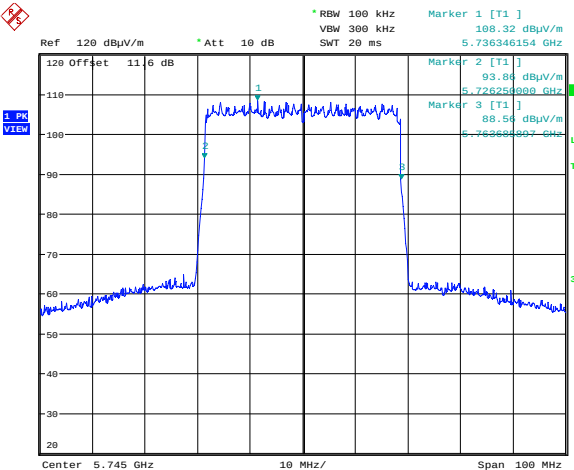
16QAM 5745 MHz
