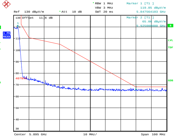
64QAM
