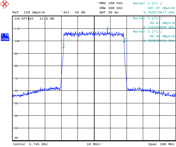
64QAM 5745 MHz
