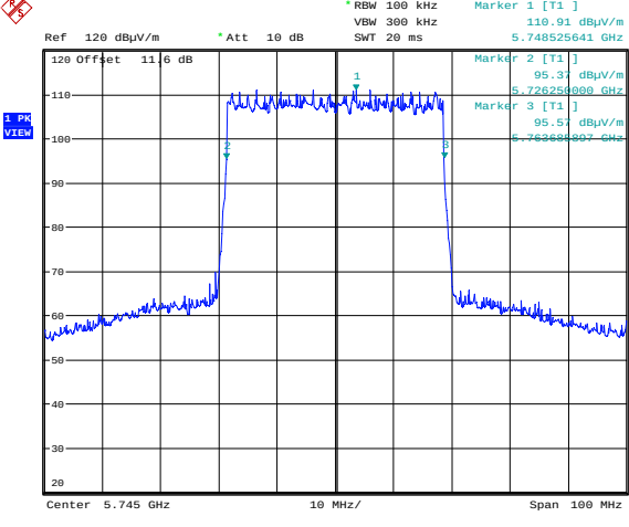
256QAM 5745 MHz
