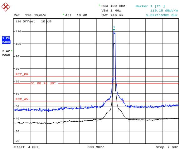
4 GHz – 7 GHz
