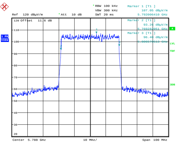
16QAM 5788 MHz
