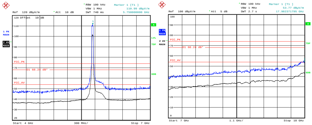
4 GHz – 7 GHz
