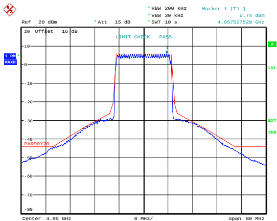
Date: 3.JAN.2003 15:58:33 Emission Mask 256 QAM; MIMO B; 4950 MHz.
