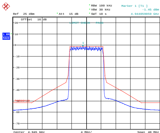
Emission Mask 16 QAM; MIMO A; 4945 MHz.
