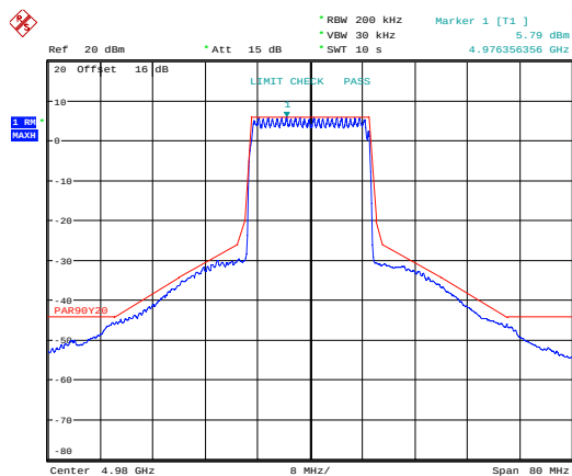
Emission Mask 64 QAM; MIMO B; 4980 MHz.
