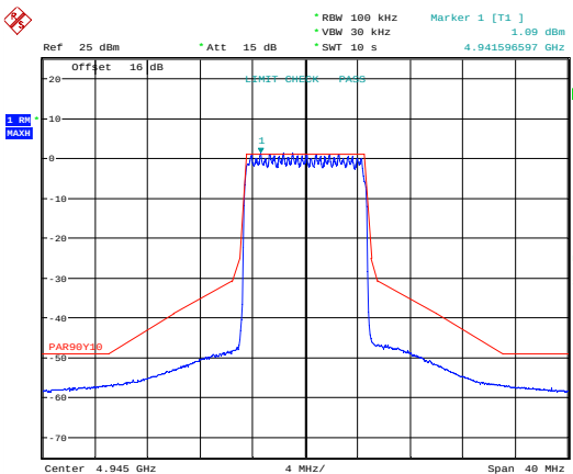
Emission Mask QPSK; MIMO B; 4945 MHz.
