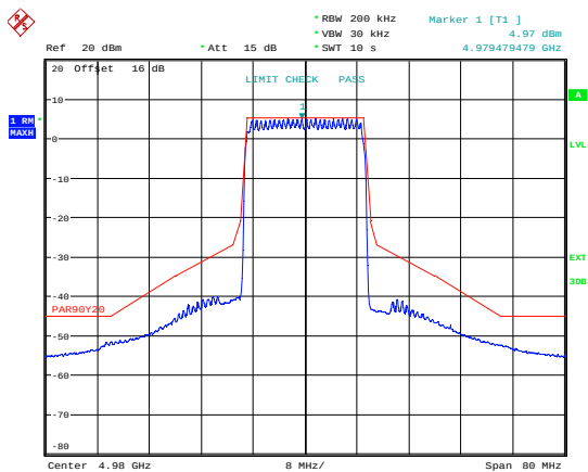
Emission Mask 16 QAM; MIMO A; 4980 MHz.
