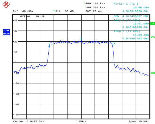
99 % Bandwidth 16 QAM; 4942.5 MHz; MIMO B.
