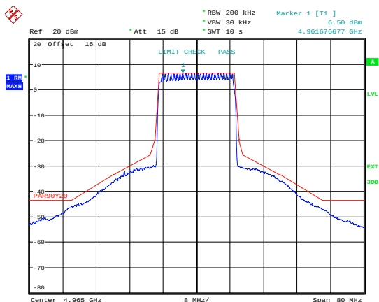
Date: 3.JAN.2003 16:12:59 Emission Mask QPSK; MIMO A; 4965 MHz.
