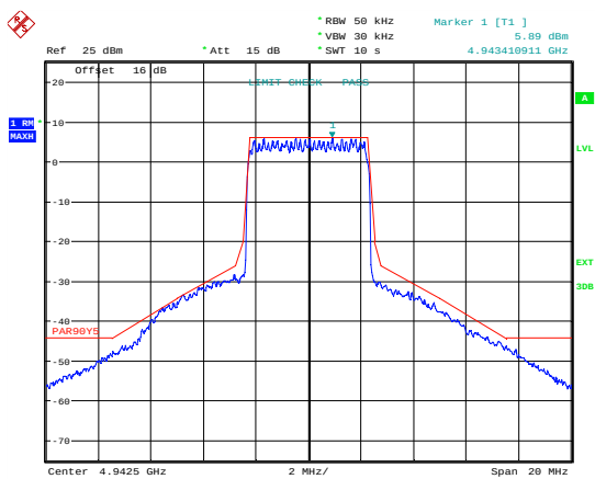
Emission Mask 16 QAM; MIMO B; 4942.5 MHz.
