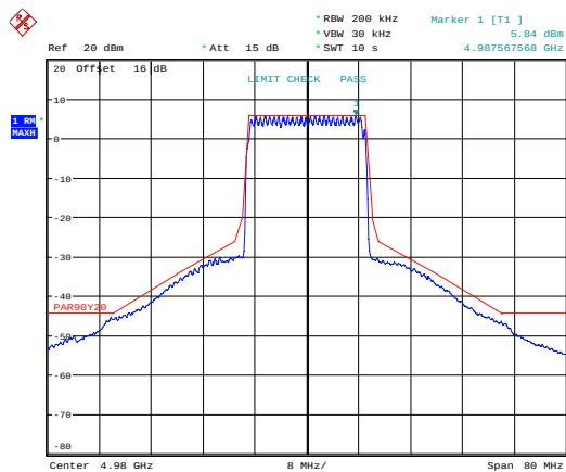
Emission Mask 16 QAM; MIMO B; 4980 MHz.
