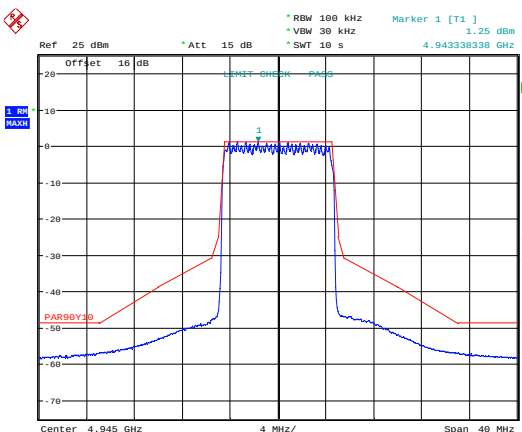
Emission Mask 16 QAM; MIMO B; 4945 MHz.
