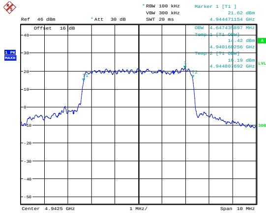
99 % Bandwidth 16 QAM; 4942.5 MHz; MIMO A.
