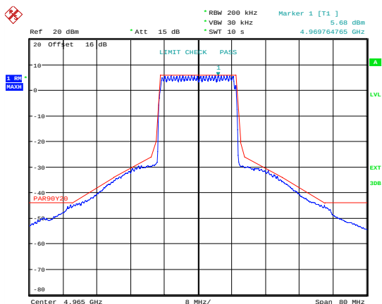
Date: 3.JAN.2003 16:11:35 Emission Mask QPSK; MIMO B; 4965 MHz.
