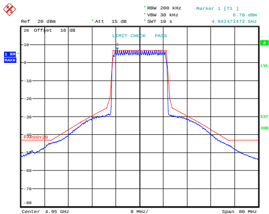
Date: 3.JAN.2003 15:48:43 Emission Mask 256 QAM; MIMO A; 4950 MHz.
