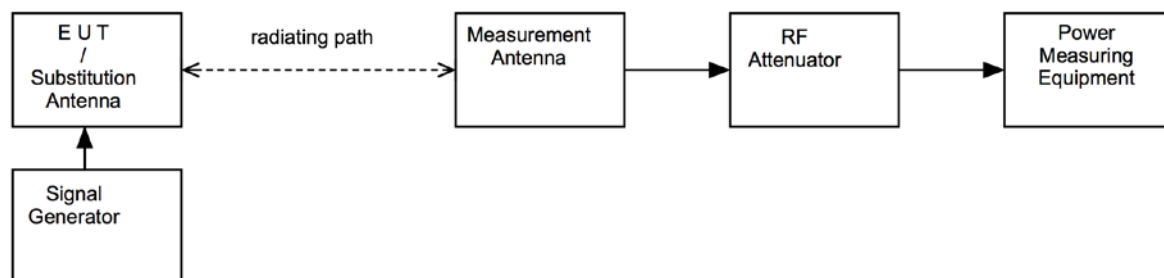
Figure v Test Setup
