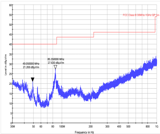
30 MHz – 1 GHz
