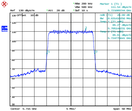
64QAM 5715 MHz
