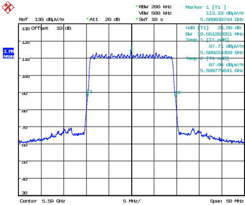
64QAM 5590 MHz
