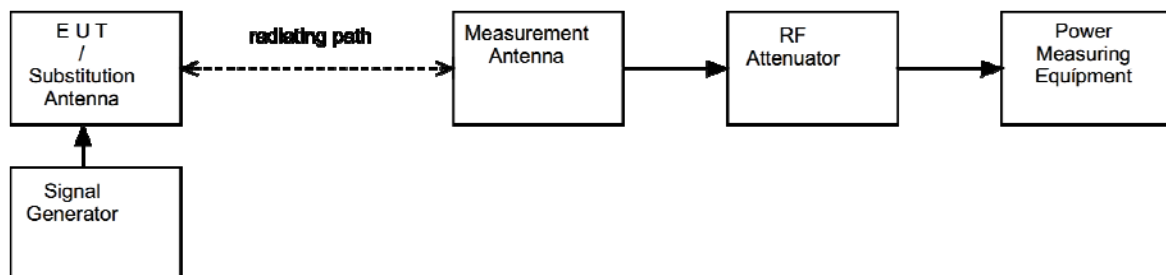
Figure iv Test Setup
