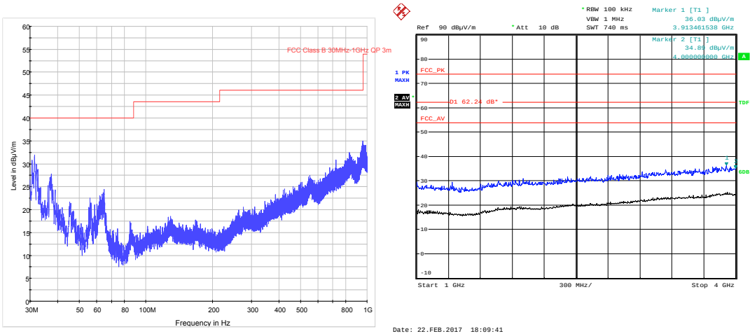
30 MHz – 1 GHz
