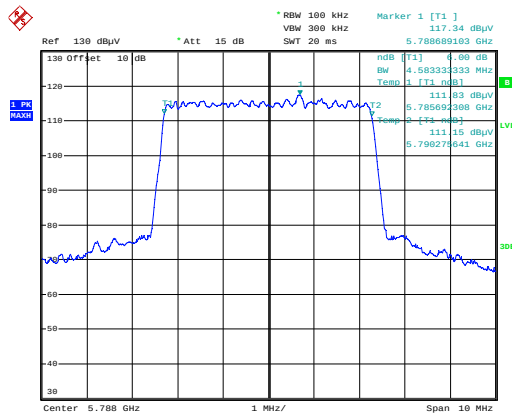
64QAM 5788 MHz
