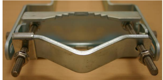
Figure 63 Assembled upper bracket connected to AP antenna
