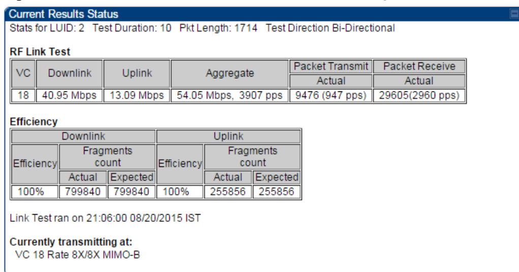
Figure 160 Link Capacity Test tab with 1714-byte packet length
