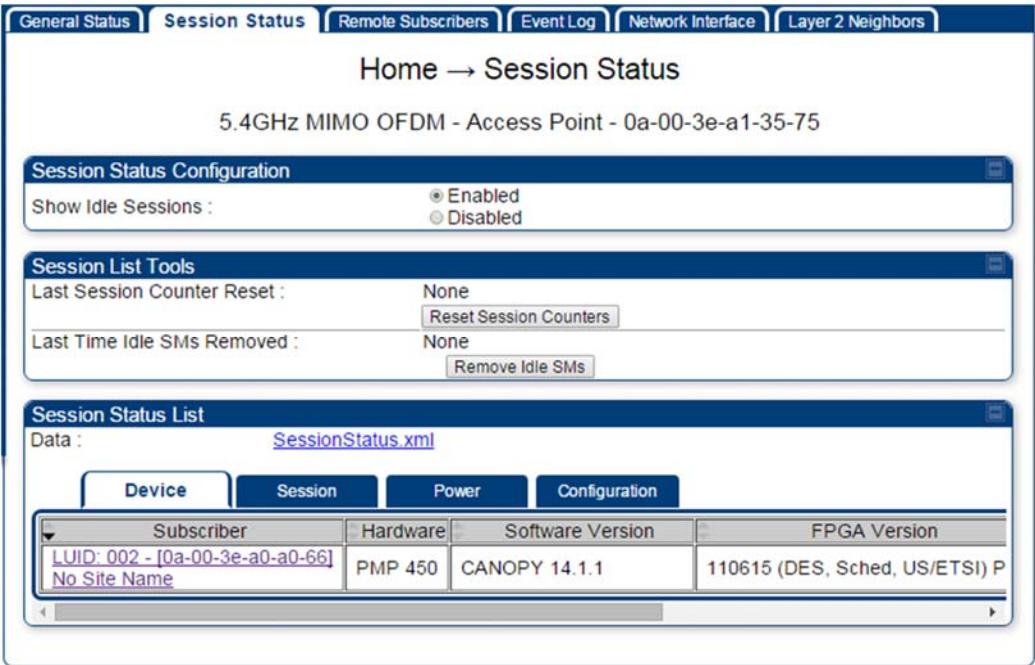
Figure 127 Session Status tab of AP
