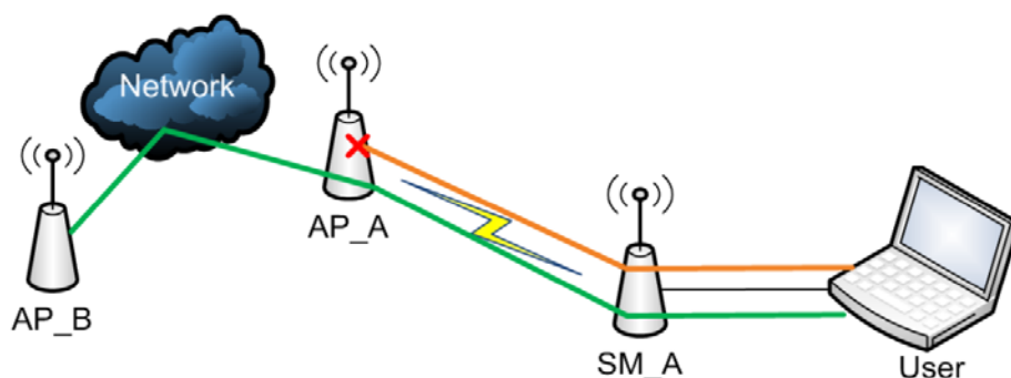
Figure 141 RF Telnet Access Restriction (orange) and Potential Security Hole (green)
