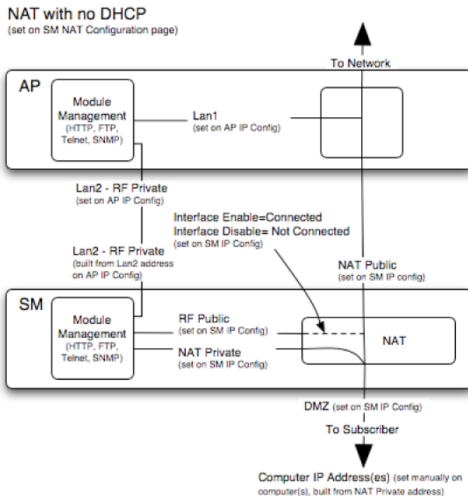
Figure 132 NAT without DHCP implementation
