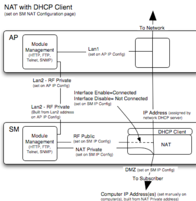
Figure 130 NAT with DHCP client implementation
