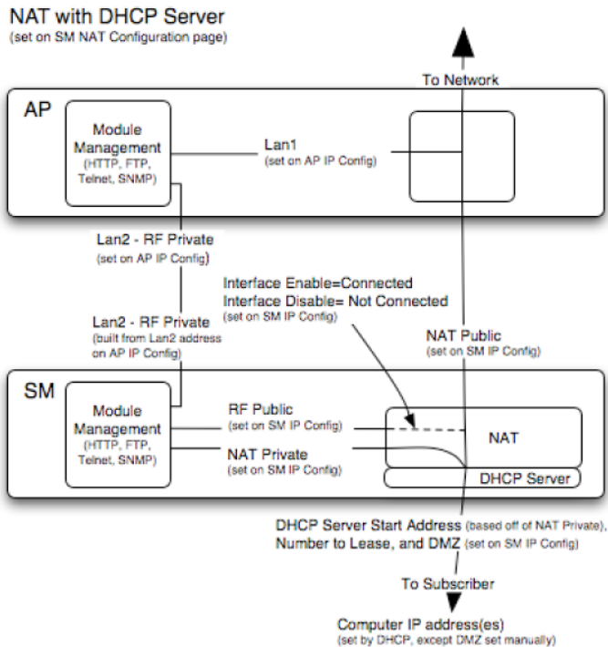
Figure 131 NAT with DHCP server implementation
