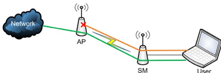
Figure 140 RF Telnet Access Restrictions (orange) and Flow through (green)
