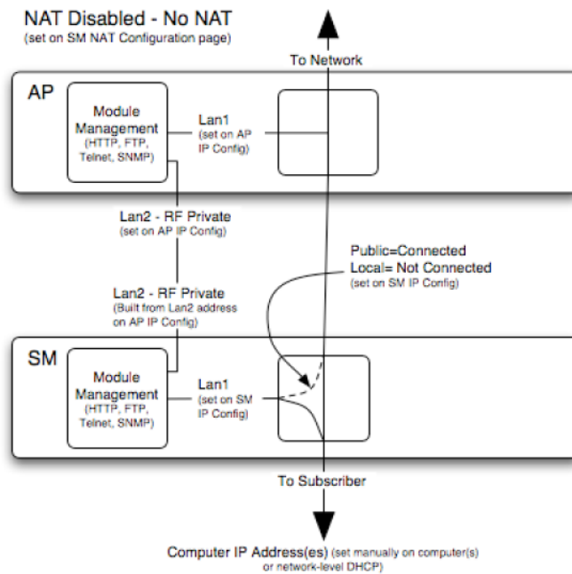
Figure 128 NAT disabled implementation
