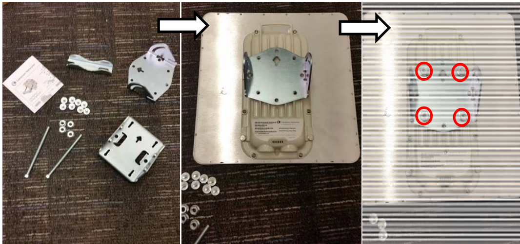
Figure 115 Fixing the mounting plate to the back of the ODU
