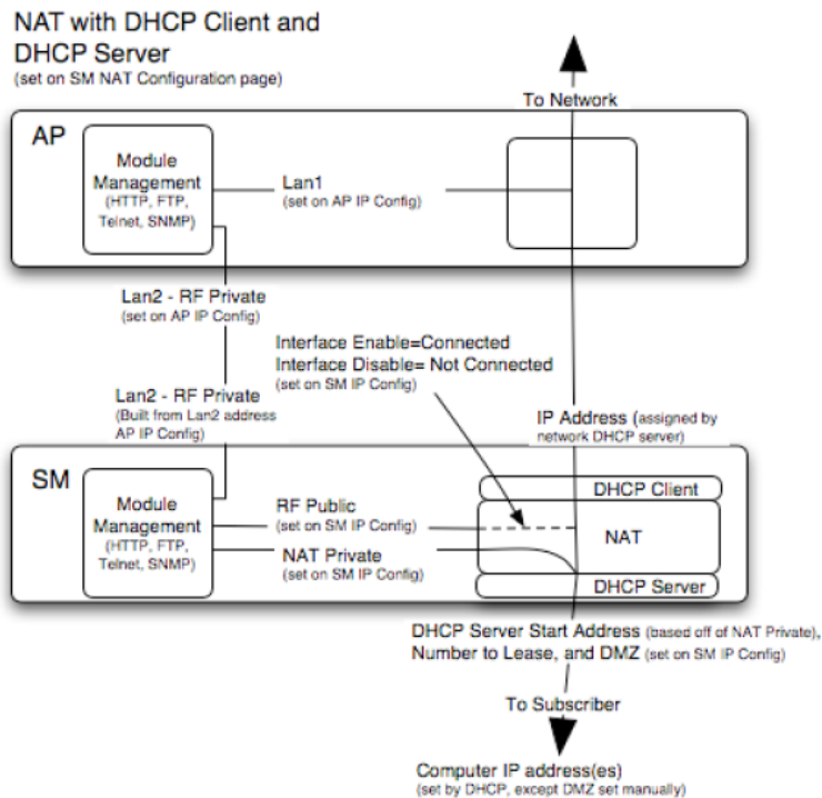
Figure 129 NAT with DHCP client and DHCP server implementation
