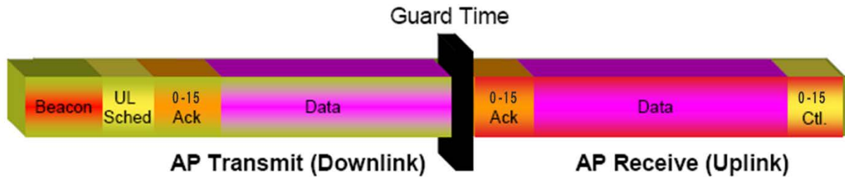
Figure 29 Frame structure
