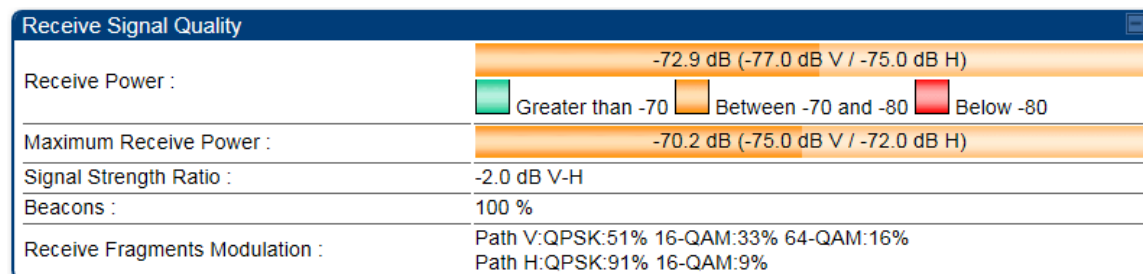
Figure 70 Alignment Tool tab of SM - Receive Power Level between -70 to -80 dBm
