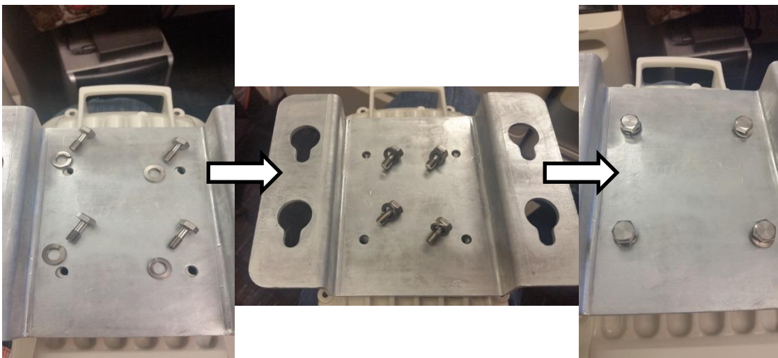
Figure 58 Attaching antenna plate to the AP
