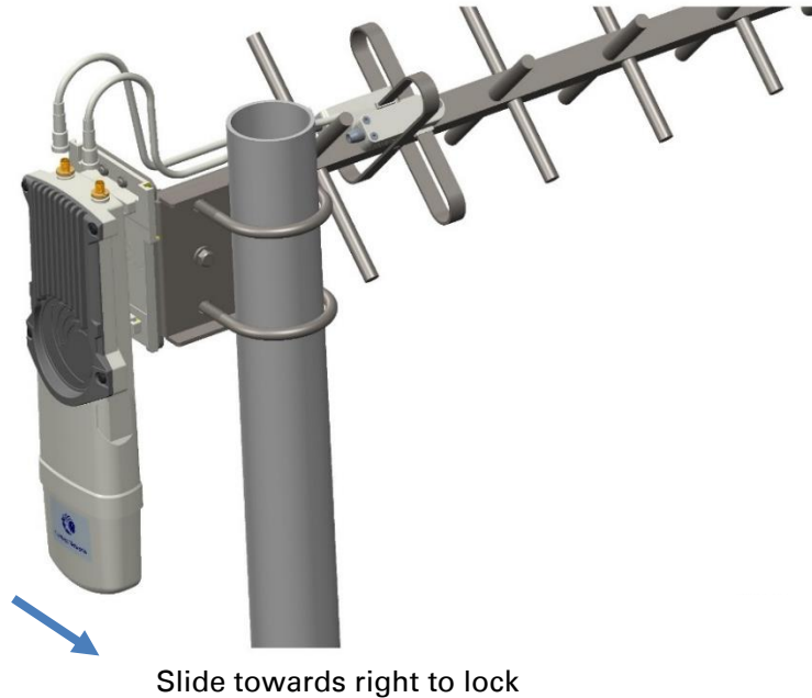
Figure 88 Fixing the radio to the antenna
