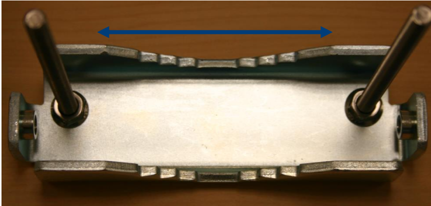
Figure 69 AP antenna upper bracket assembly
