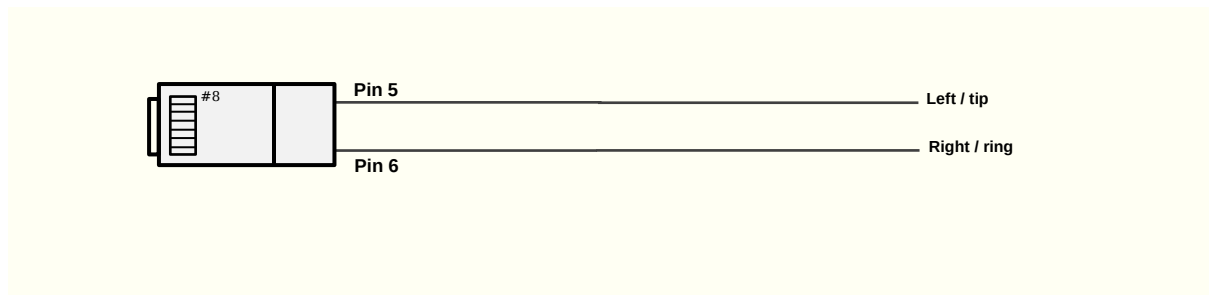
Figure 22 RJ12 Alignment Tone Cable
