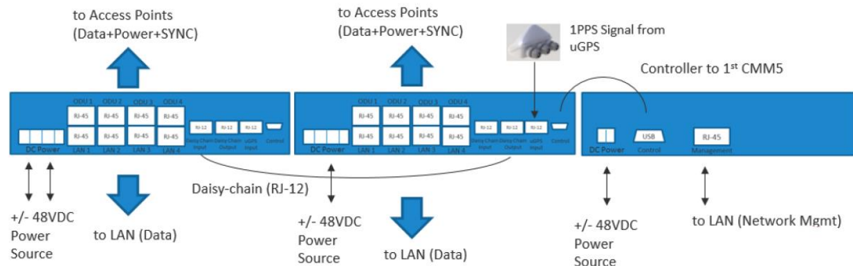
Figure 27 Cluster Management: Scenario 2 CMM5 Controller
