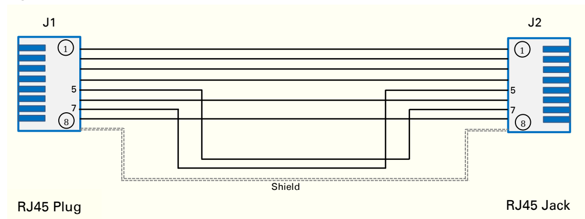
Figure 32 CMM4 power adapter cabling diagram
