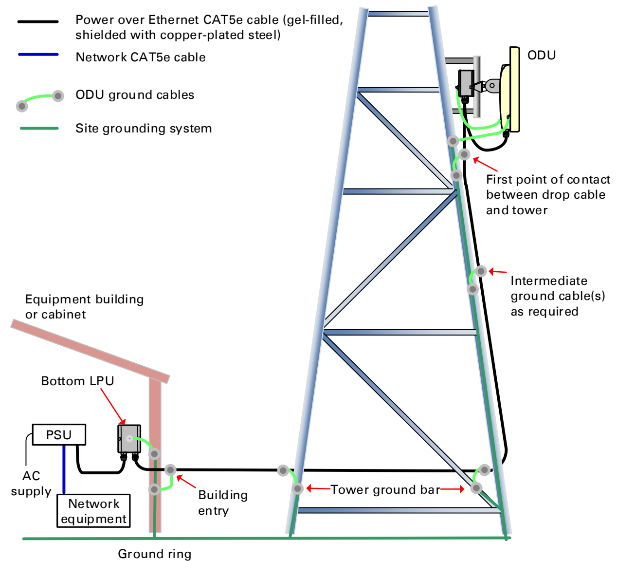
Figure 37 Mast or tower installation
