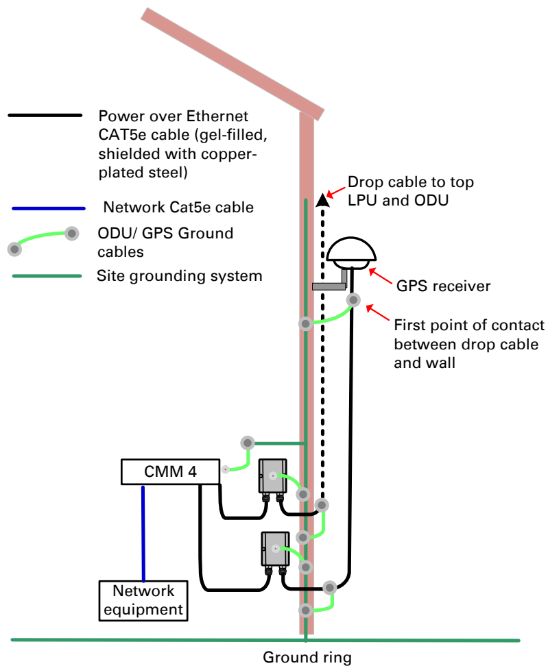
Figure 40 GPS receiver wall installation
