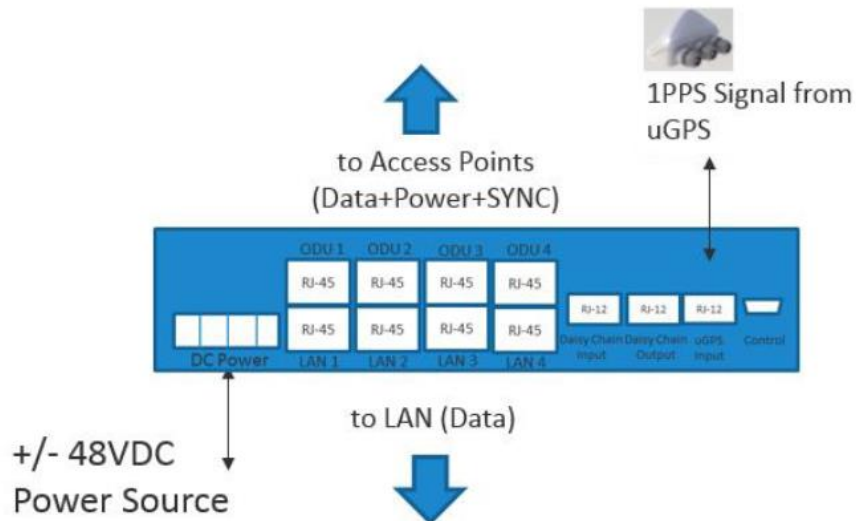
Figure 26 CMM5 Controller Cluster Management: Scenario 1
