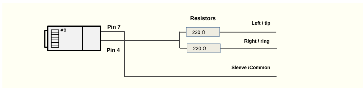
Figure 21 Alignment Tone Cable
