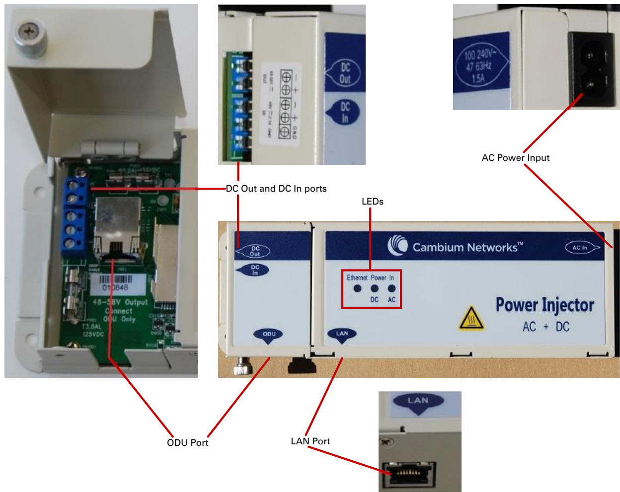
Figure 12 AC+DC Enhanced Power Injector interfaces
