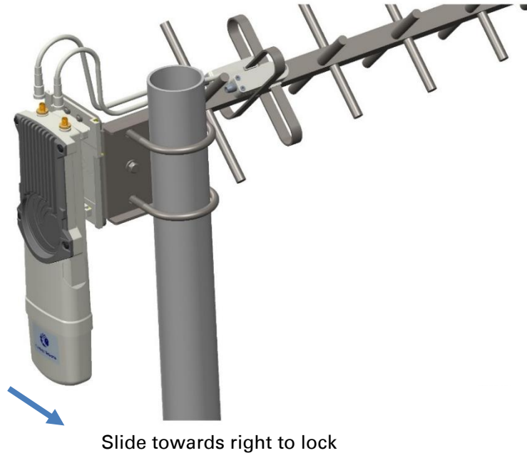
Figure 95 Fixing the radio to the antenna
