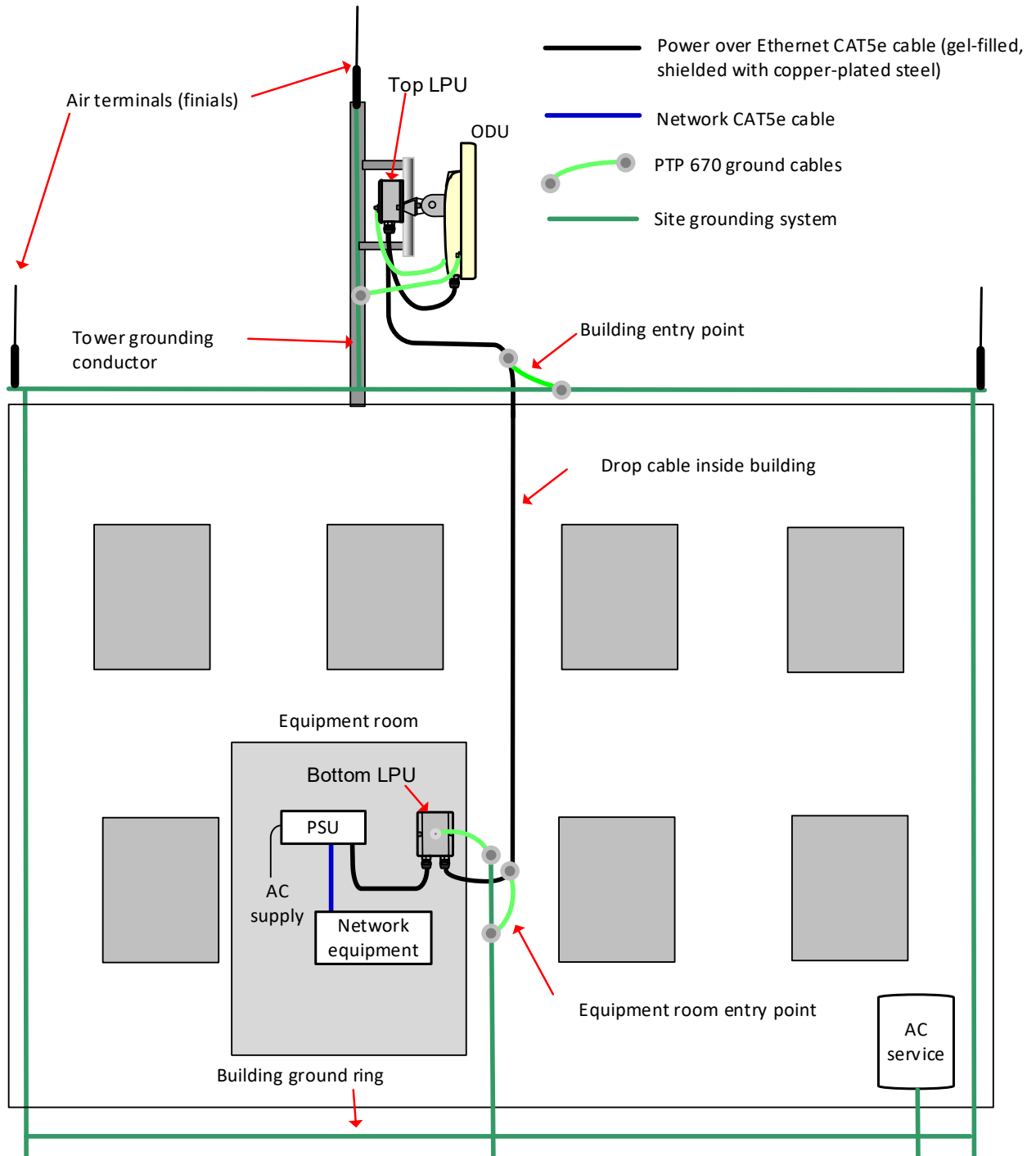
Figure 38 Roof installation
