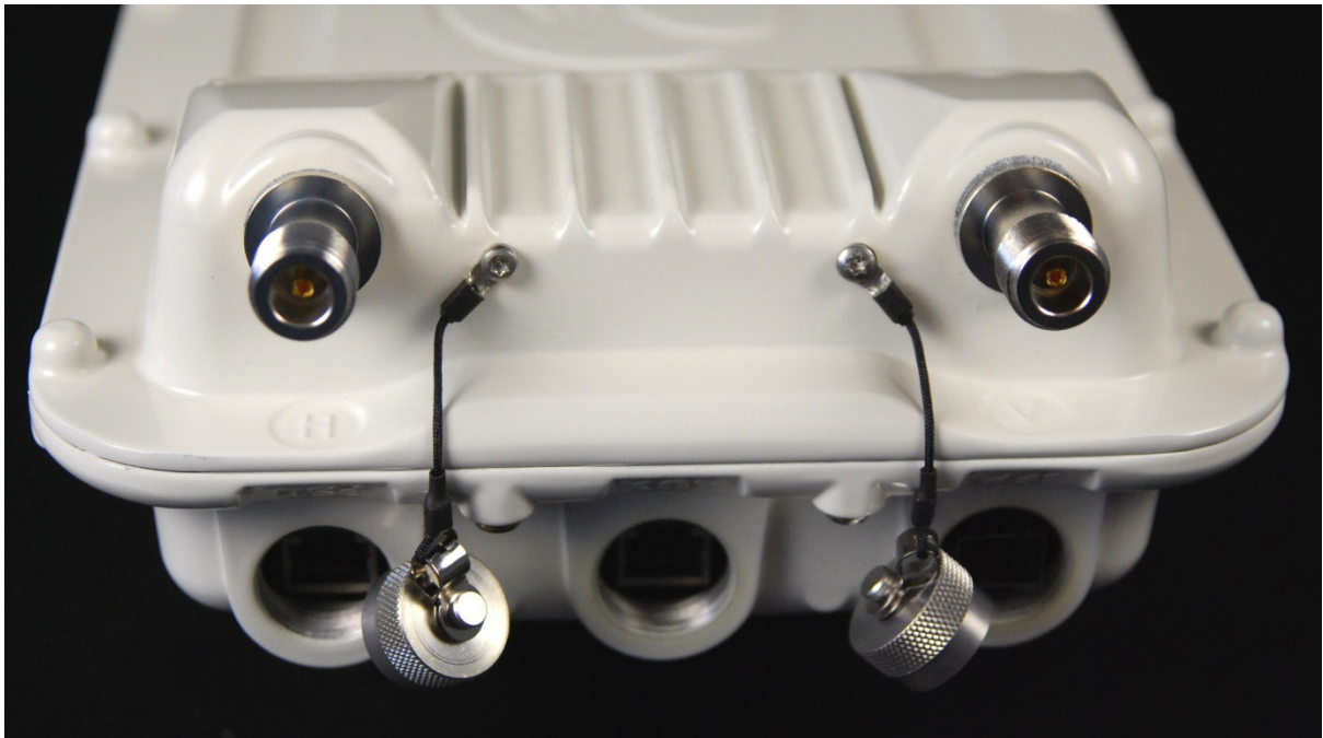
Bottom View C050067B014A - PTP 670 (4.9 to 5.9 GHz) ATEX/HAZLOC Connectorized ODU (FCC) – RF 'N' Type Connector Covers Removed
