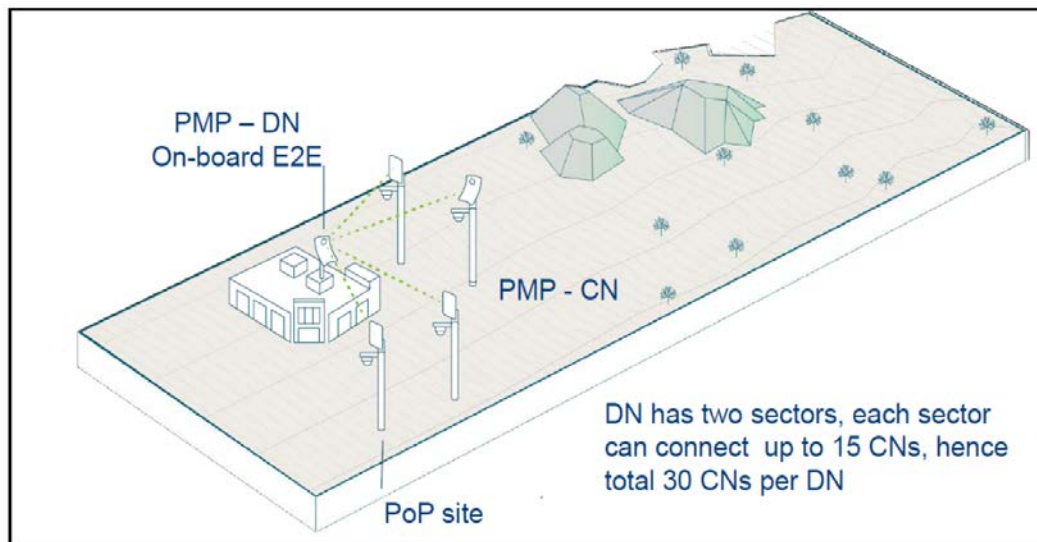
Figure 8: PMP Topology
