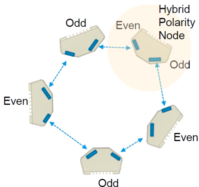
Figure 56: Hybrid polarity
