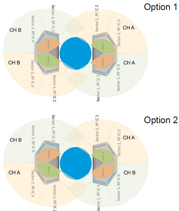
Figure 55: When two V5000 devices are co-located at the same site
