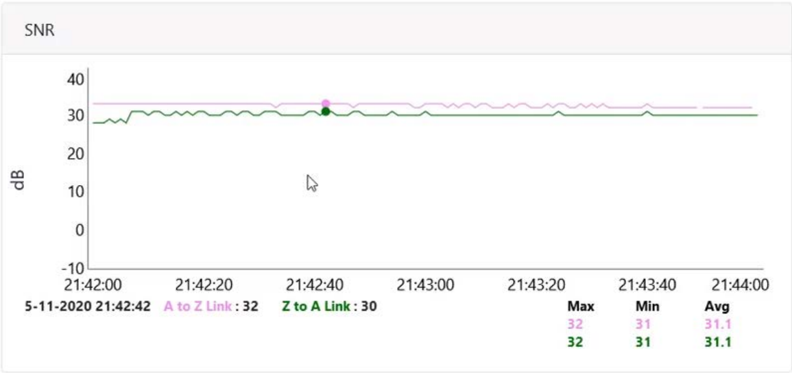
Figure 10 : SNR graph
