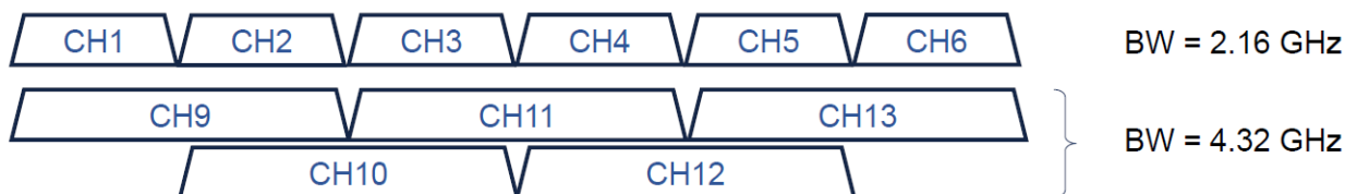
Figure 1 : Frequency bands
