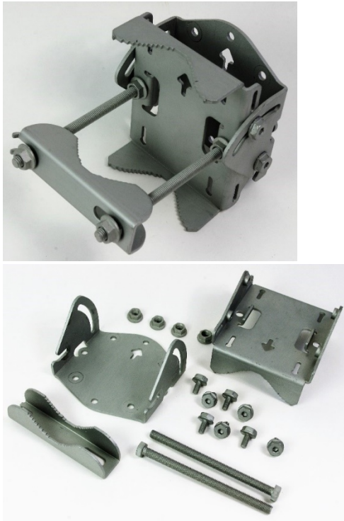
Figure 6: Tilt Bracket Assembly
