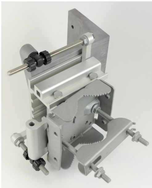
Figure 9: Precision Bracket
