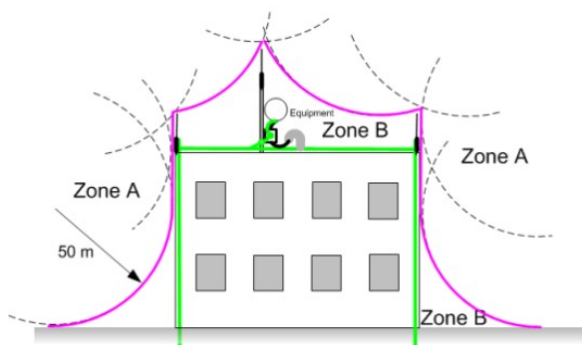
Figure 26 : Rolling sphere method to determine the lightning protection zones
