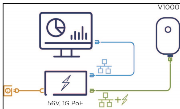
Figure 127: V1000 powering diagram
