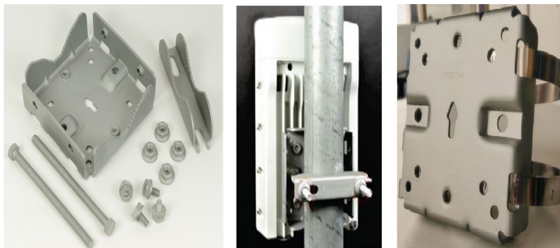
Figure 23: Pole mount
