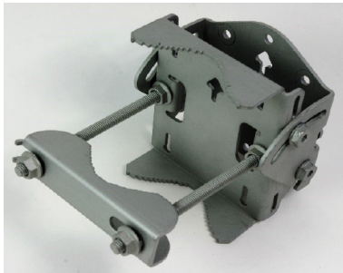
Figure 22 : Tilt bracket assembly
