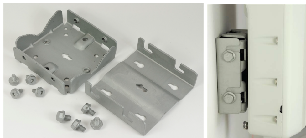
Figure 24: Wall mount
