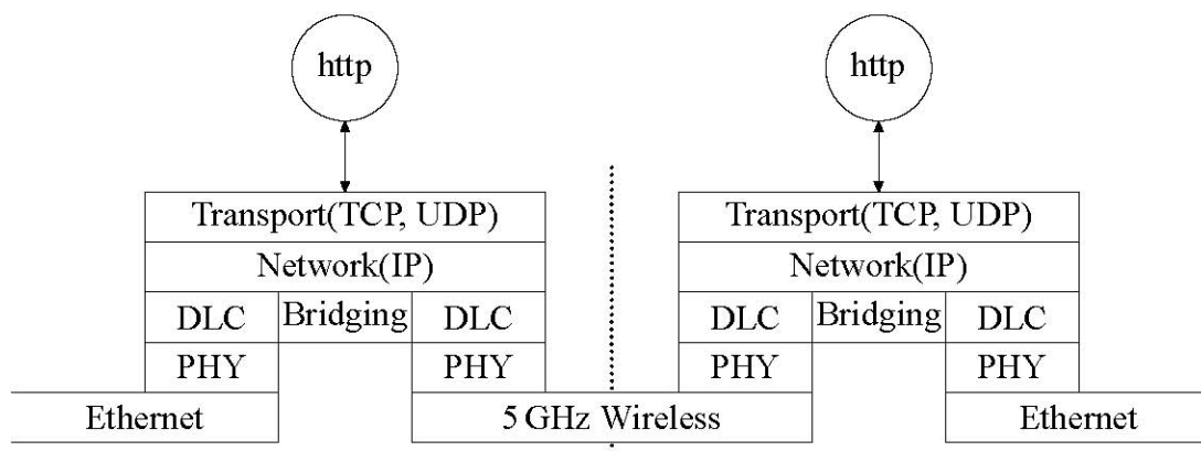
Figure 6 OS-Gemini Layer Diagram
