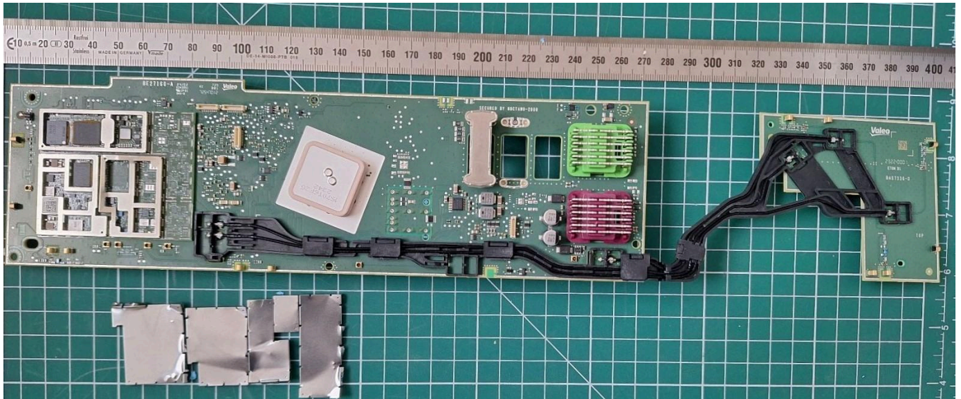
int_top_Unshielded
