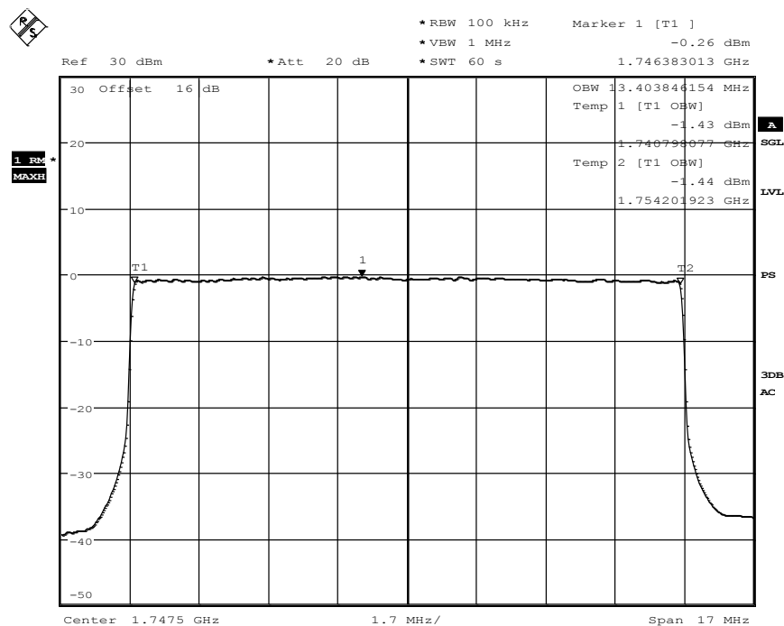
Diagram 35.413, QPSK-Modulation
