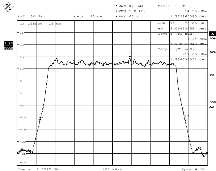
Diagram 34.404, QPSK-Modulation
