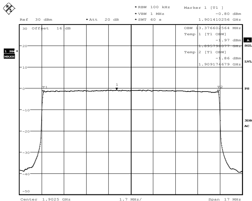
Diagram 35.212, QPSK-Modulation
