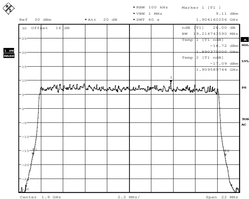
Diagram 34.217, QPSK-Modulation
