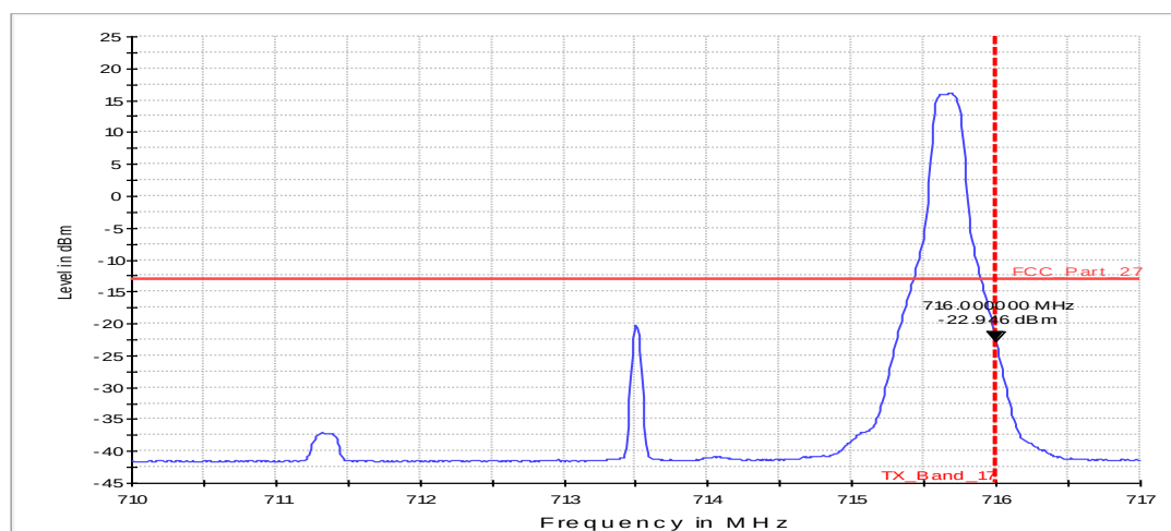
Fula2_003b_FCC_27_BE_high_Channel_23825_BW_5MHz_AV
