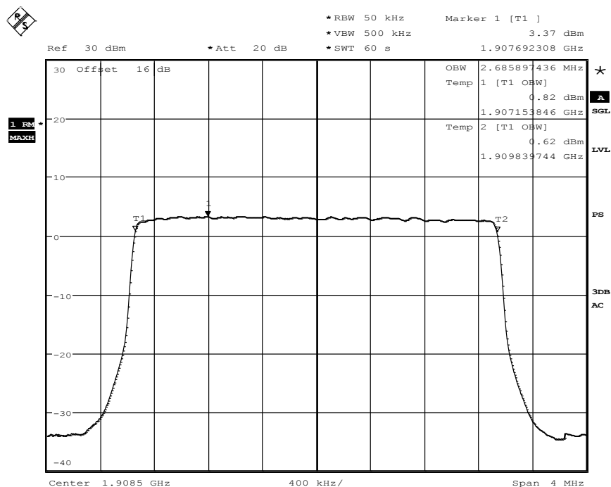
Diagram 35.203, QPSK-Modulation
