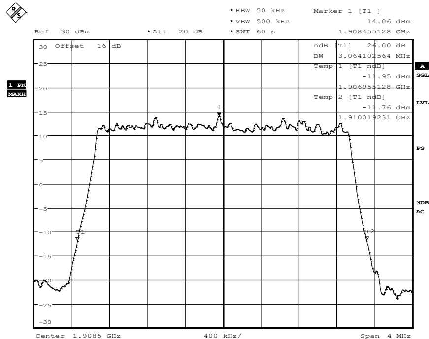
Diagram 34.203, QPSK-Modulation
