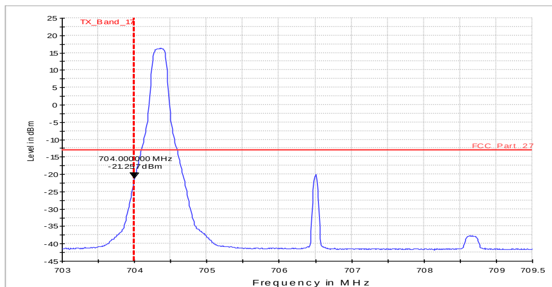
Fula2_001b_FCC_27_BE_low_Channel_23755_BW_5MHz_AV
