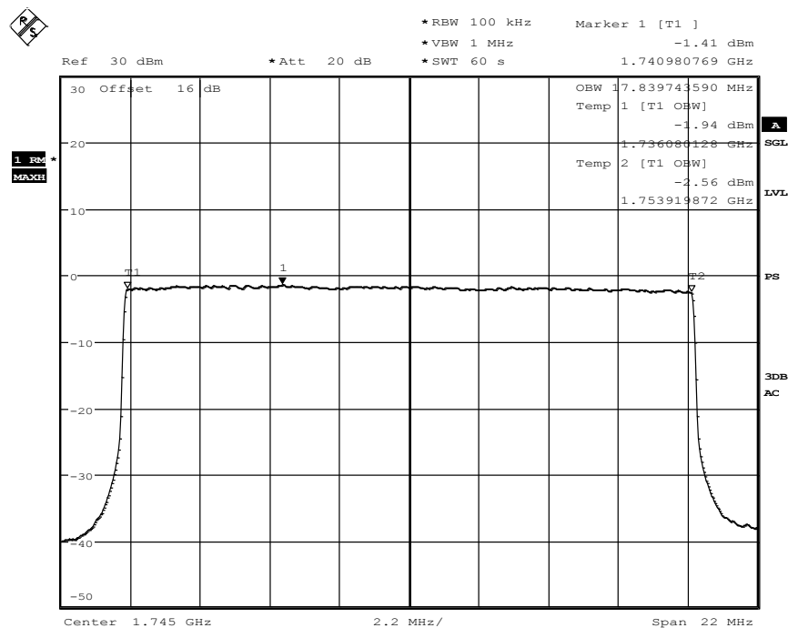
Diagram 35.418, QPSK-Modulation
