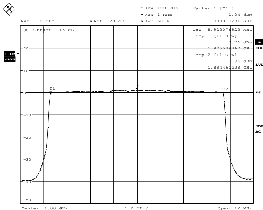
Diagram 35.209, QPSK-Modulation
