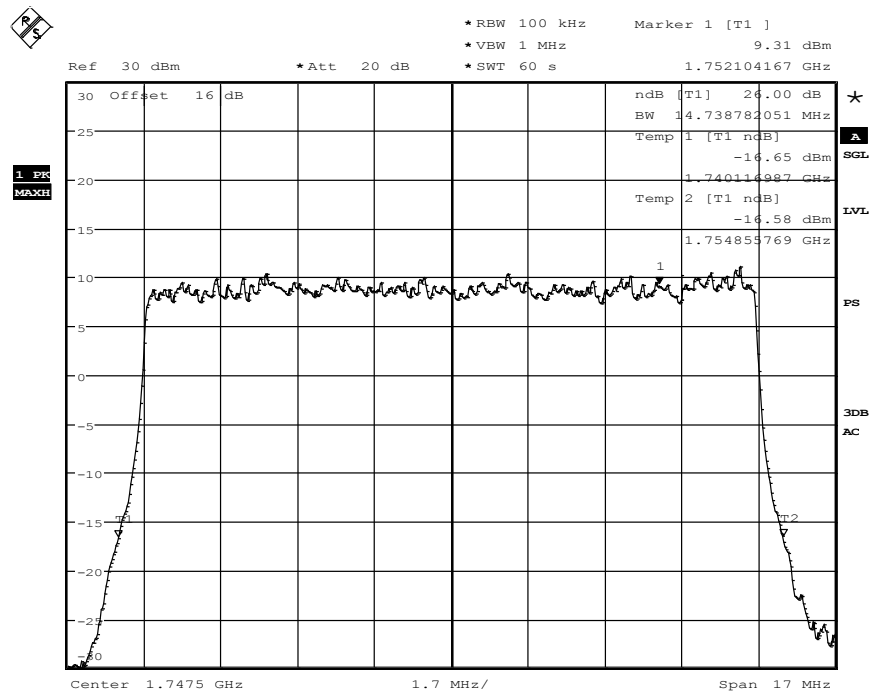
Diagram 34.413, QPSK-Modulation
