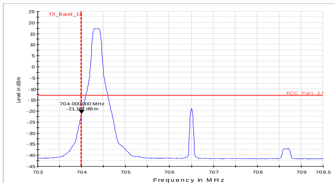
Fula2_001b_FCC_27_BE_low_Channel_23755_BW_5MHz_AV
