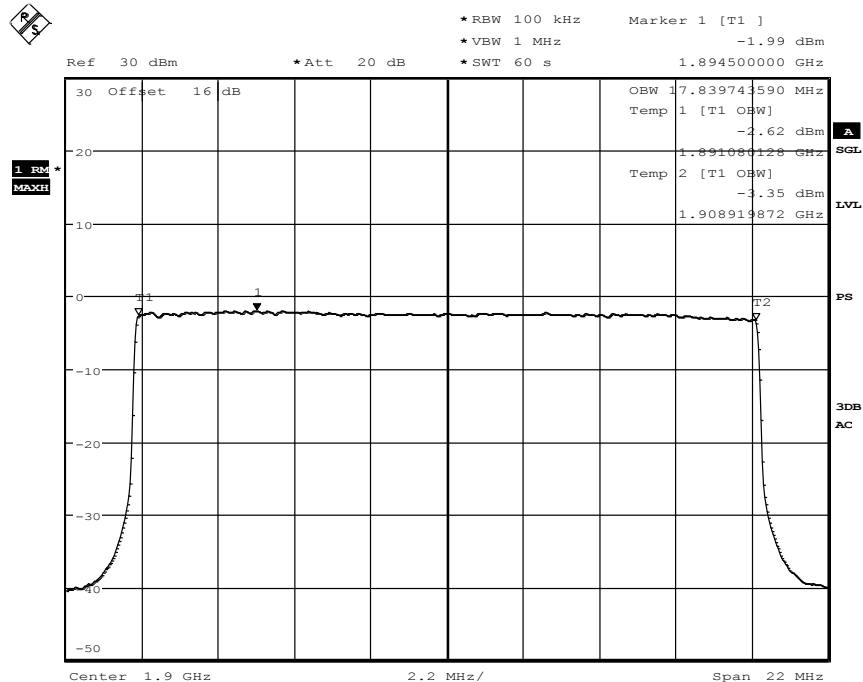
Diagram 35.217, QPSK-Modulation
