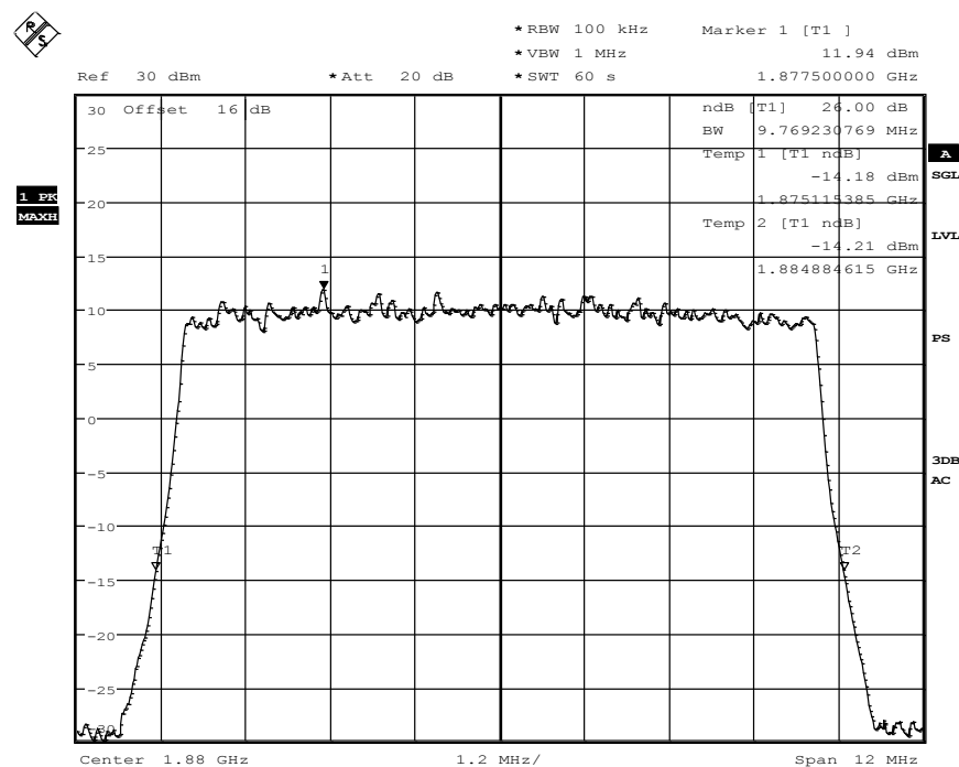
Diagram 34.209, QPSK-Modulation
