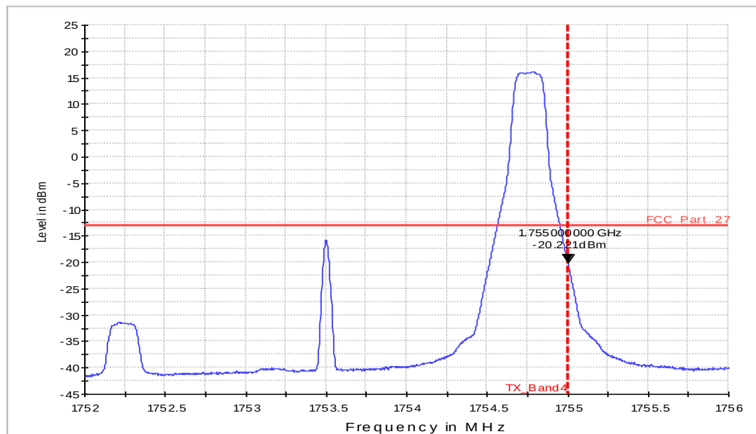
Fula2_016b_FCC_27_BE_High_Ch20385_BW_3MHz_AV
