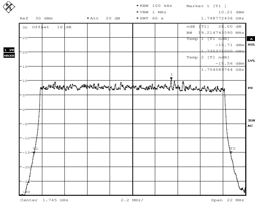
Diagram 34.418, QPSK-Modulation
