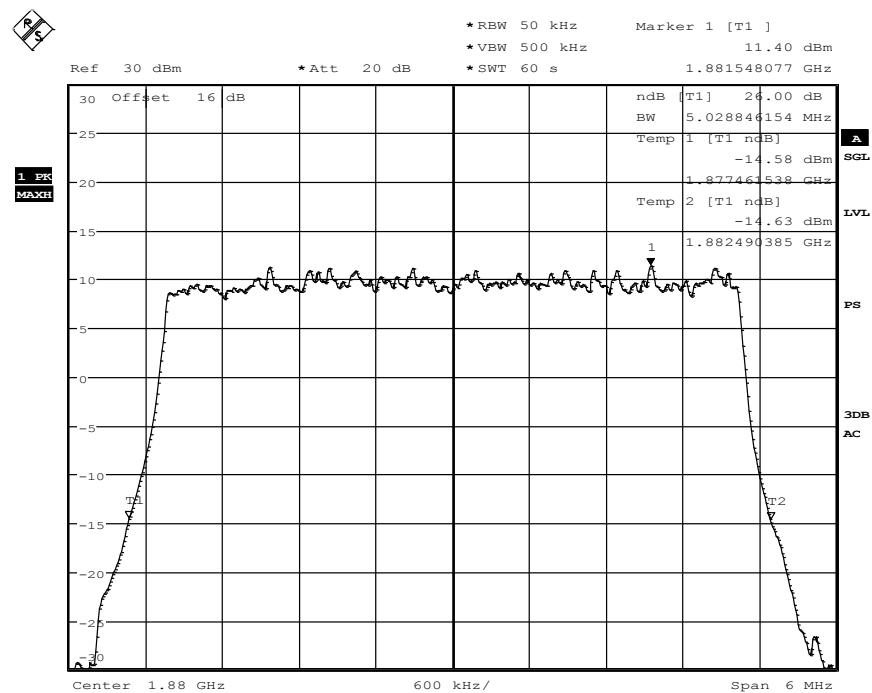
Diagram 34.207, QPSK-Modulation
