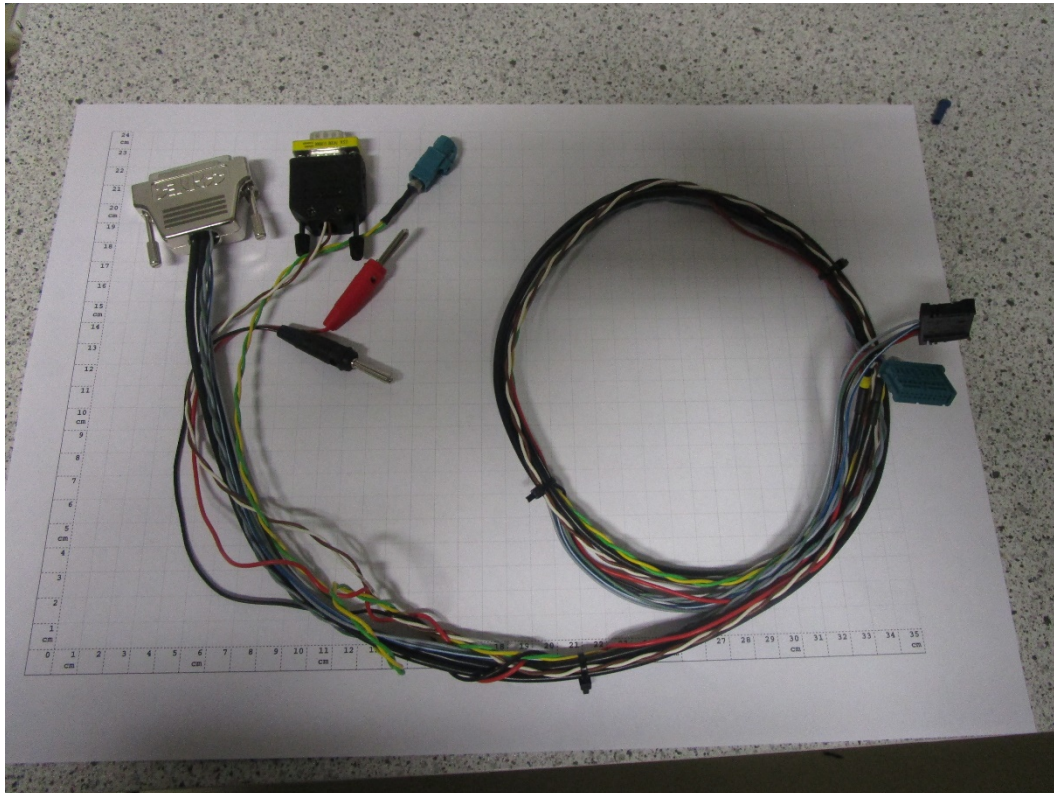
Photograph 8: Main wiring
