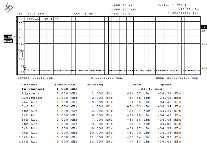
Diagram 39: 9.711b_CH21425_BW5_25RBhigh_QAM16_sweep1_intBW
