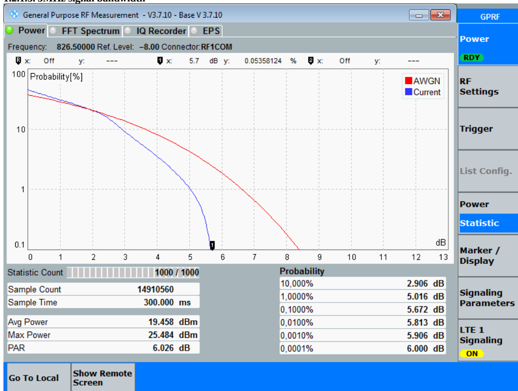
Diagram: Ch20425_QAM_12RB_5MHz
