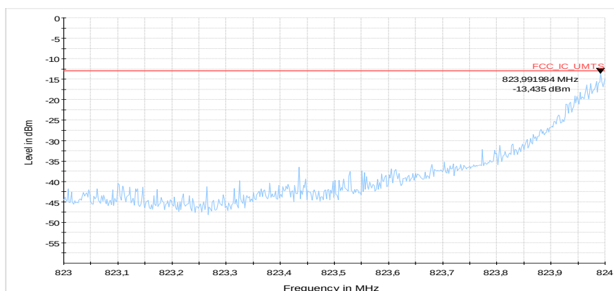
Diagram 2: 9.503b_CH20415_BW3_6RBlow_QAM
