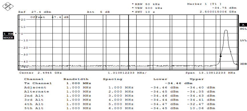
Diagram 12: 9.701b_CH20775_BW5_1RBlow_QAM_sweep1
