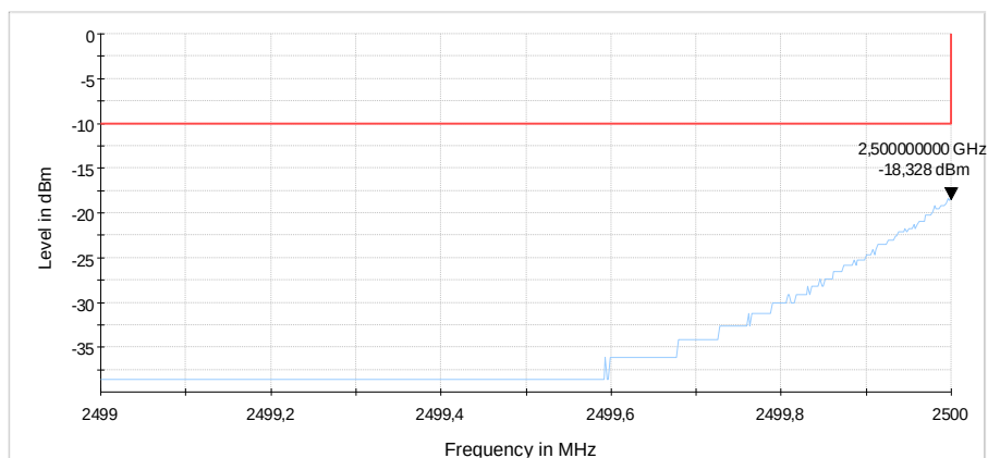
Diagram 24: 9.703b_CH20800_BW10_1RBlow_16QAM_sweep2
