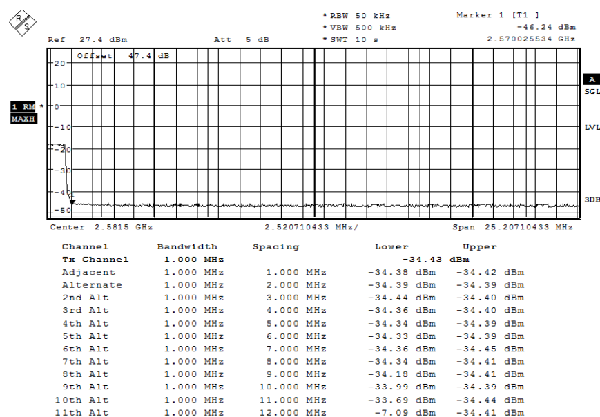
Diagram 36: 9.711a_CH21425_BW5_25RBhigh_QPSK_sweep1_intBW
