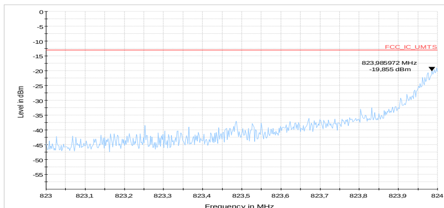
Diagram 1: 9.503a_CH20407_BW1.4_6RBlow_QAM
