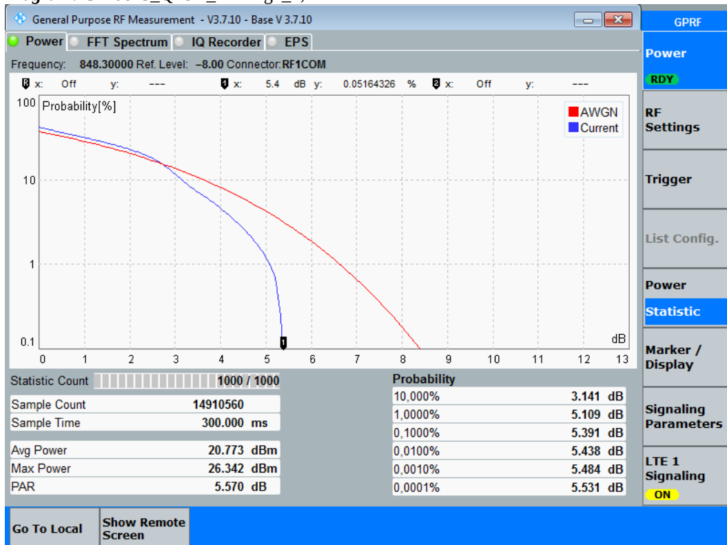
Diagram: Ch20643_QAM_1RB_low_1,4MHz
