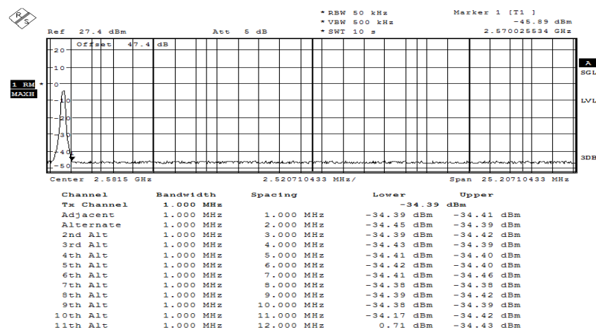
Diagram 32: 9.710b_CH21425_BW5_1RBhigh_QAM16_sweep1
