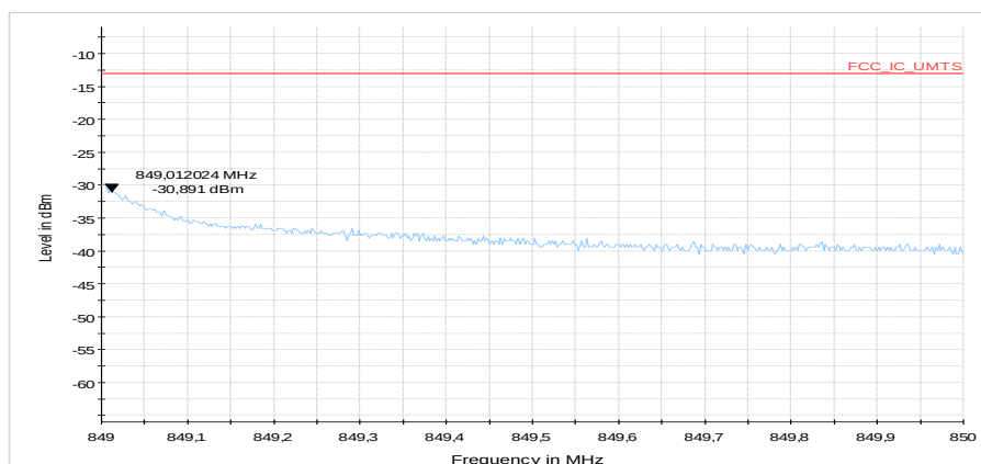
Diagram 7: 9.513a_CH20635_BW3_15RBhigh_QPSK
