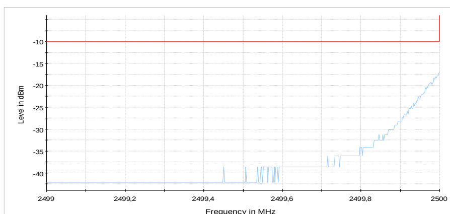
Diagram 11: 9.701a_CH20775_BW5_1RBlow_QPSK_sweep2
