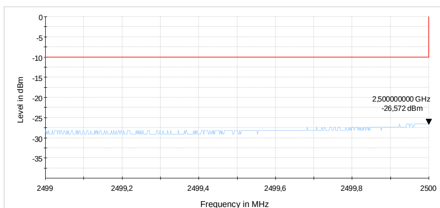
Diagram 26: 9.704a_CH20800_BW10_50RBlow_QPSK_sweep2
