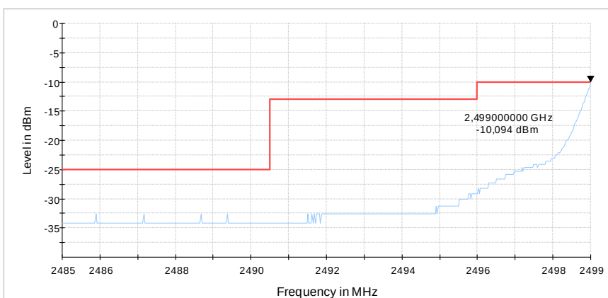
Diagram 15: 9.702a_CH20775_BW5_25RBlow_QPSK_sweep1
