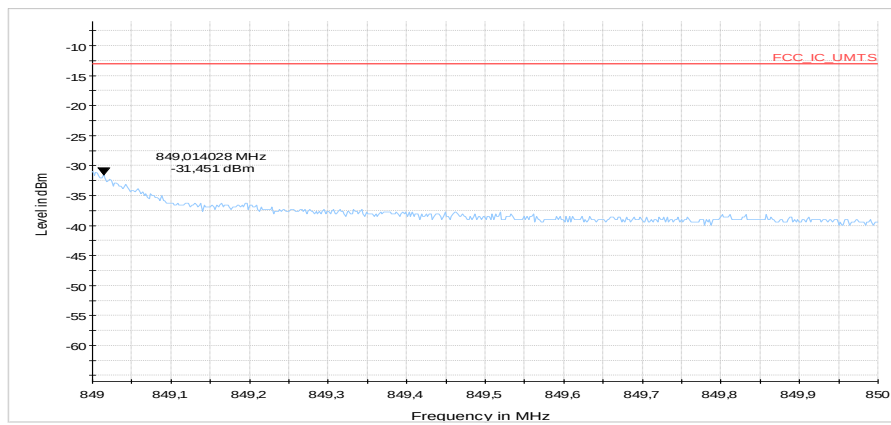
Diagram 8: 9.513b_CH20635_BW3_15RBhigh_QAM
