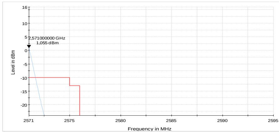
Diagram 29: 9.710a_CH21425_BW5_1RBhigh_QPSK_sweep1
