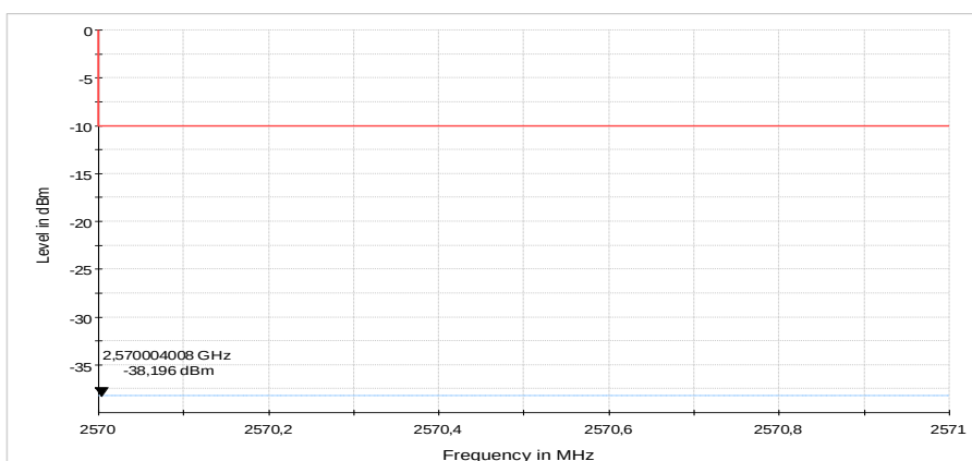
Diagram 48: 9.713b_CH21400_BW10_50RBhigh_QAM16_sweep2
