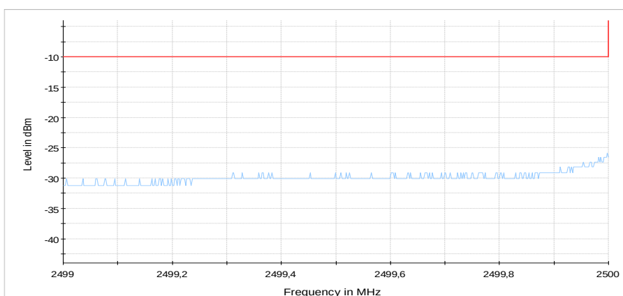
Diagram 16: 9.702a_CH20775_BW5_25RBlow_QPSK_sweep2
