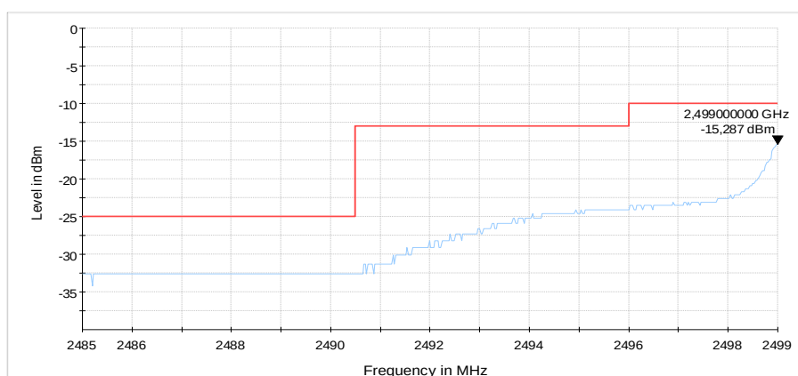
Diagram 25: 9.704a_CH20800_BW10_50RBlow_QPSK_sweep1
