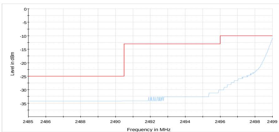
Diagram 17: 9.702b_CH20775_BW5_25RBlow_QAM_sweep1
