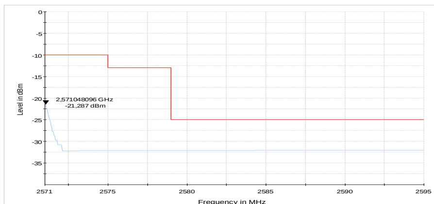
Diagram 43: 9.712b_CH21400_BW10_1RBhigh_QAM_sweep1
