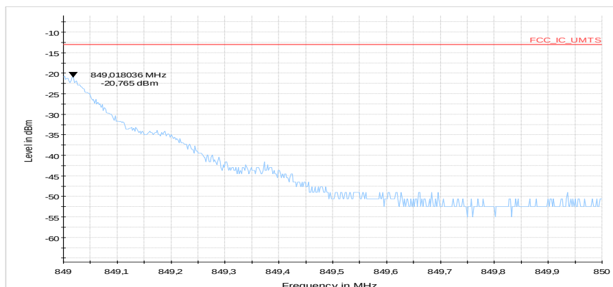
Diagram 5: 9.512a_CH20635_BW3_1RBhigh_QPSK
