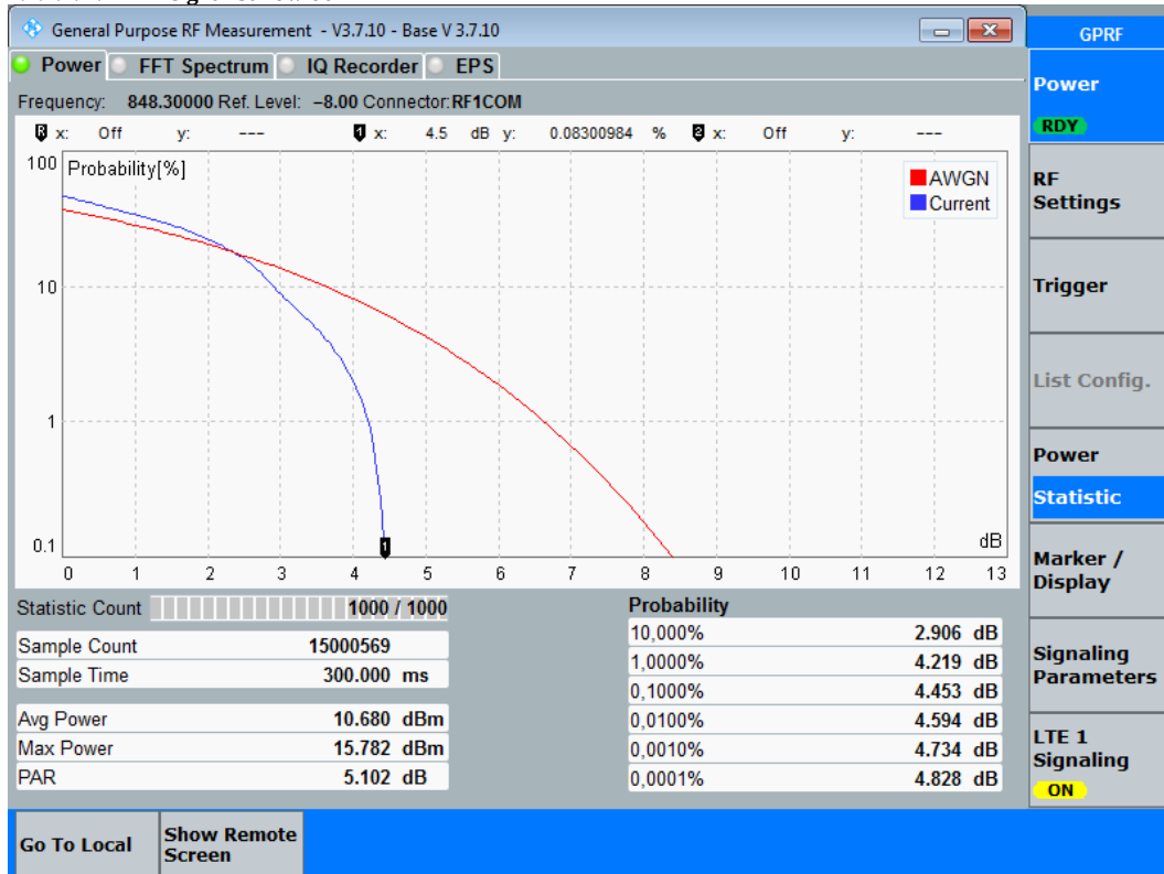
Diagram: Ch20643_QPSK_1RBhigh_1,4MHz
