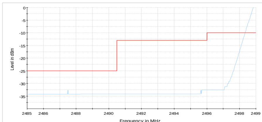
Diagram 9: 9.701a_CH20775_BW5_1RBlow_QPSK_sweep1
