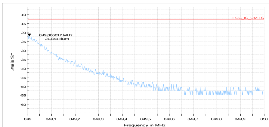
Diagram 6: 9.512b_CH20635_BW3_1RBhigh_QAM
