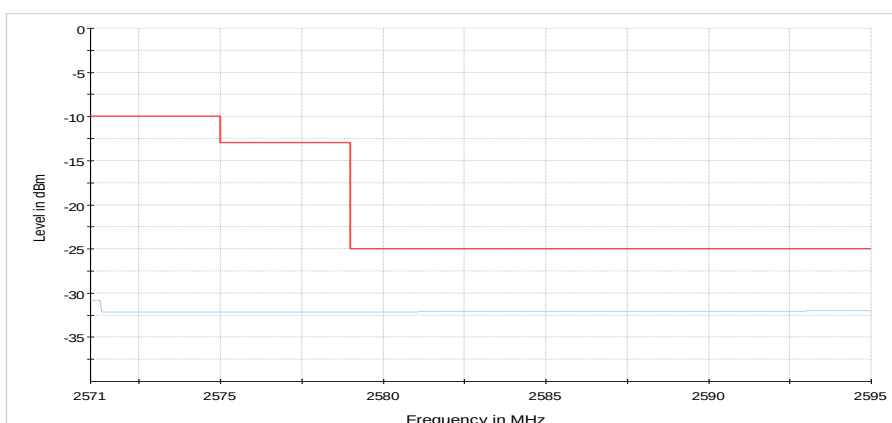
Diagram 47: 9.713b_CH21400_BW10_50RBhigh_QAM16_sweep1
