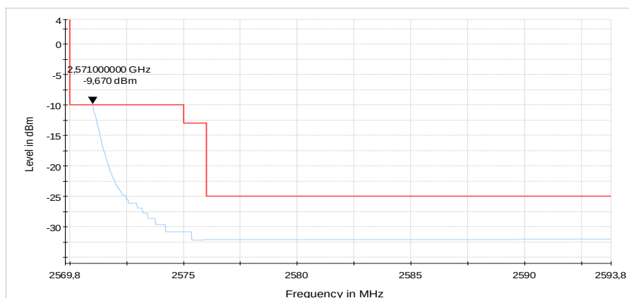
Diagram 38: 9.711b_CH21425_BW5_25RBhigh_QAM16_sweep1
