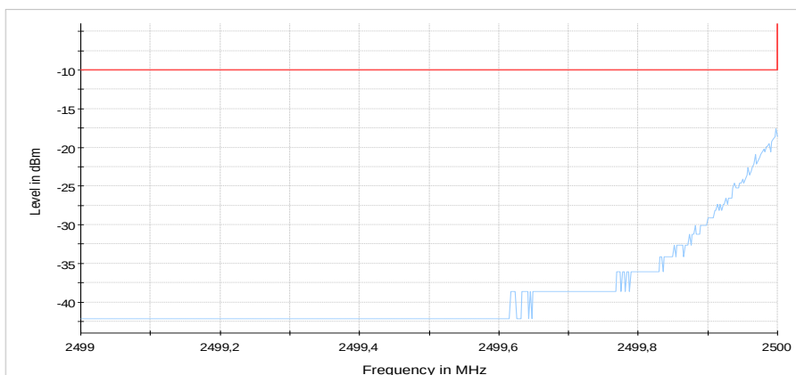
Diagram 14: 9.701b_CH20775_BW5_1RBlow_QAM_sweep2
