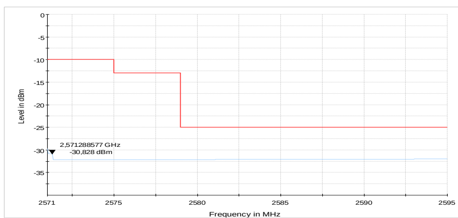
Diagram 45: 9.713a_CH21400_BW10_50RBhigh_QPSK_sweep1
