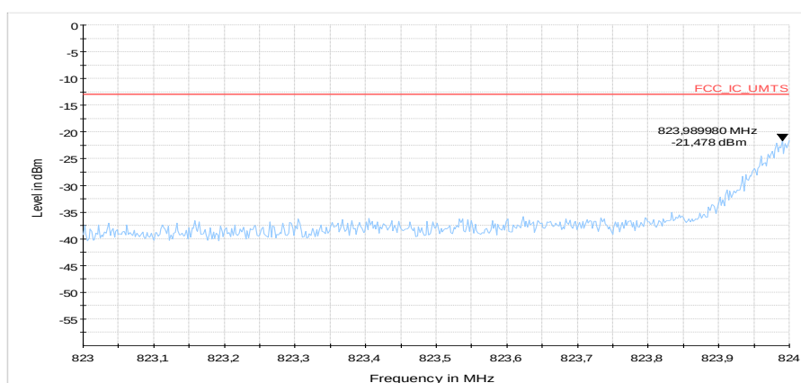
Diagram 3: 9.504a_CH20415_BW3_15RBlow_QPSK
