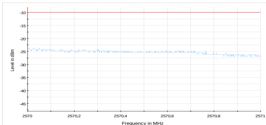
Diagram 37: 9.711a_CH21425_BW5_25RBhigh_QPSK_sweep2
