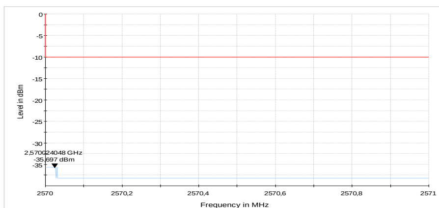
Diagram 44: 9.712b_CH21400_BW10_1RBhigh_QAM16_sweep2
