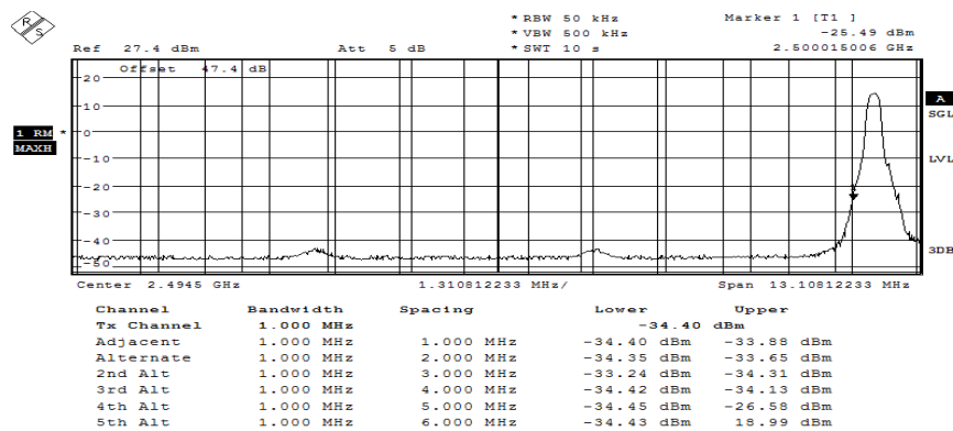
Diagram 29: 9.710a_CH21425_BW5_1RBhigh_QPSK_sweep1
