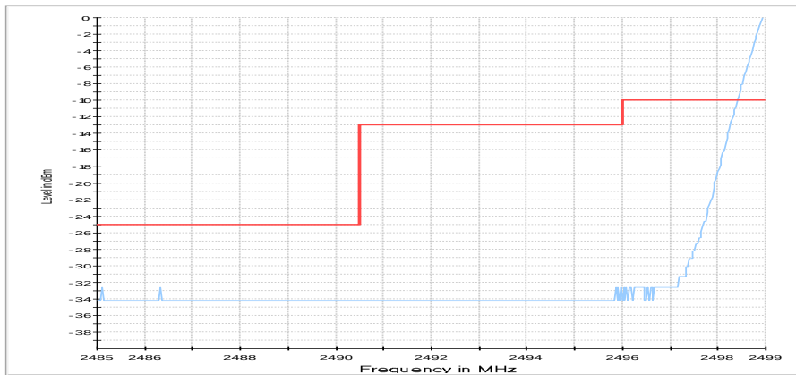
Diagram 12: 9.701b_CH20775_BW5_1RBlow_QAM_sweep1
