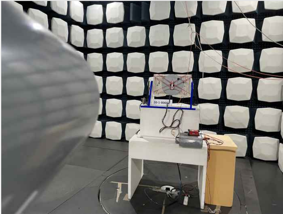
Photograph 1: EUT Test Setup in the anechoic chamber, Radiated emissions
