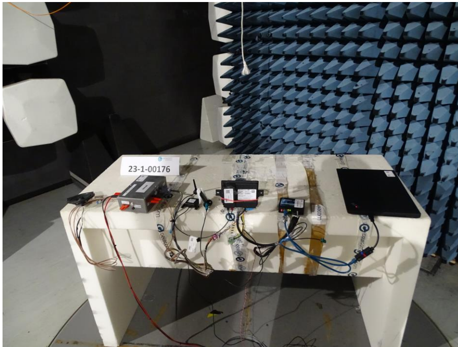
Photograph 3 : Radiated Emission below 1 GHz, close up view
