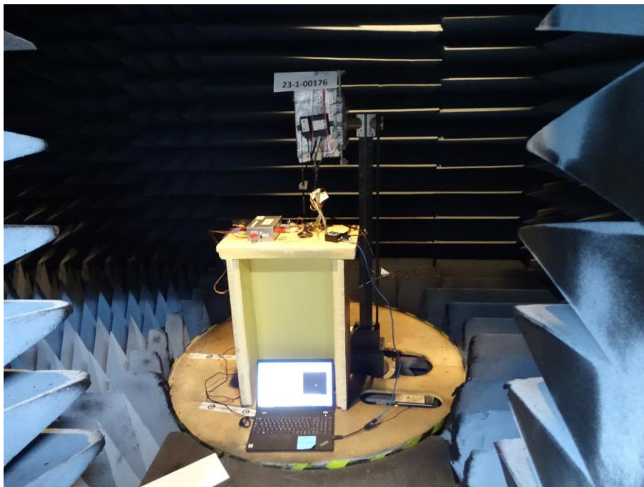
Photograph 6 : Radiated Emission above 1 GHz, overall view
