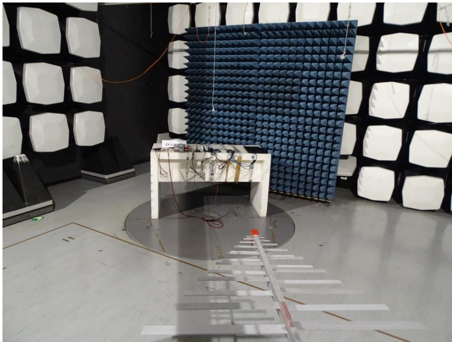
Photograph 2 : Radiated Emission below 1 GHz, overall view
