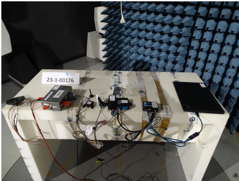
Photograph 1 : Radiated Emission below 1 GHz, close up view
