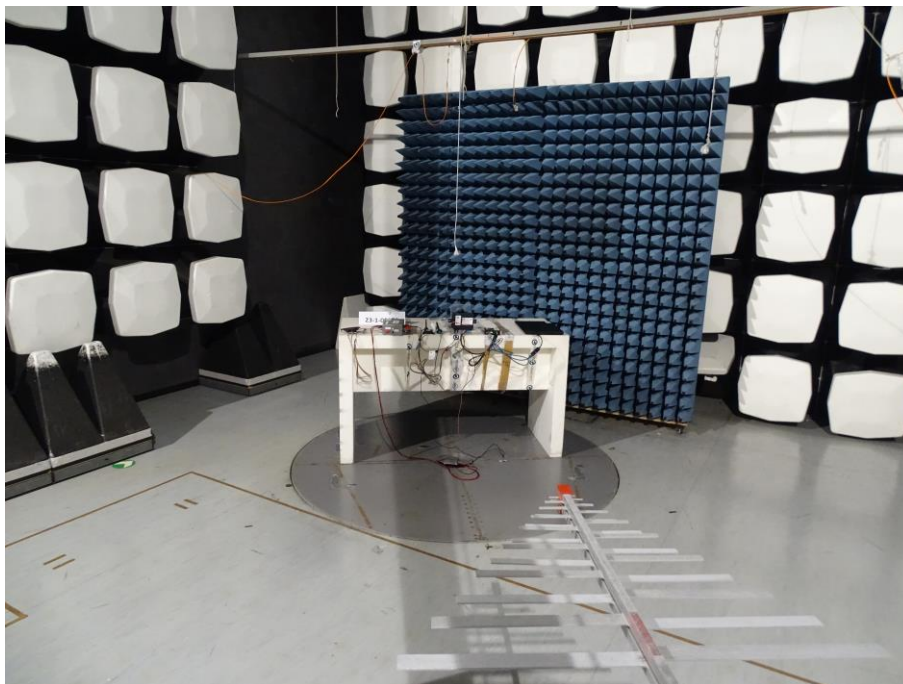
Photograph 4 : Radiated Emission below 1 GHz, overall view
